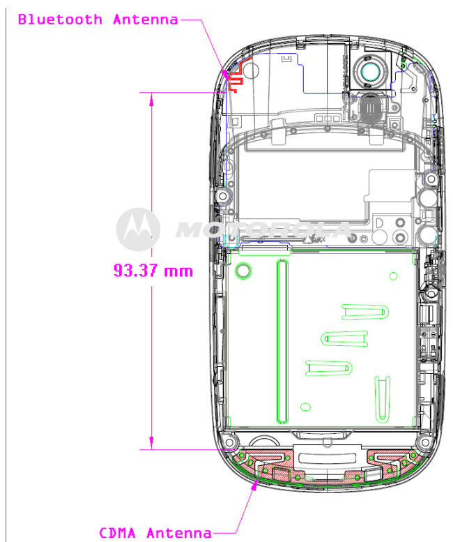
Figure 2: Antenna Separation Distance
