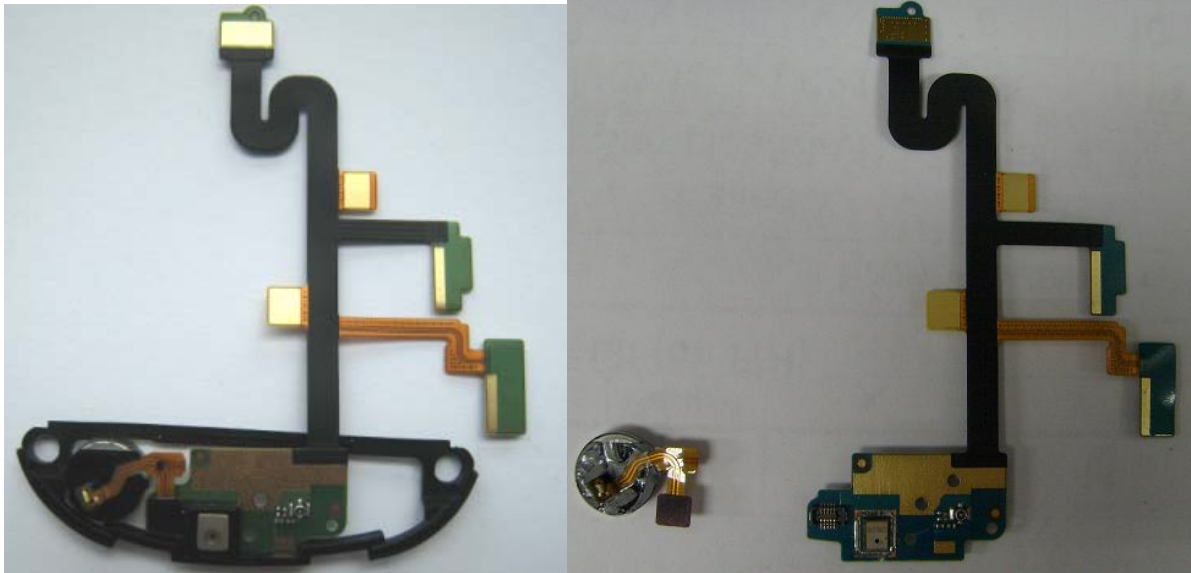
Linear Acoustic PCB Bottom W/ Shield Vibrator Acoustic PCB Bottom W/O Shield
