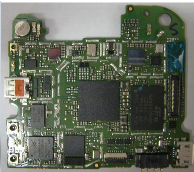
Main Board Top W/O Shields
