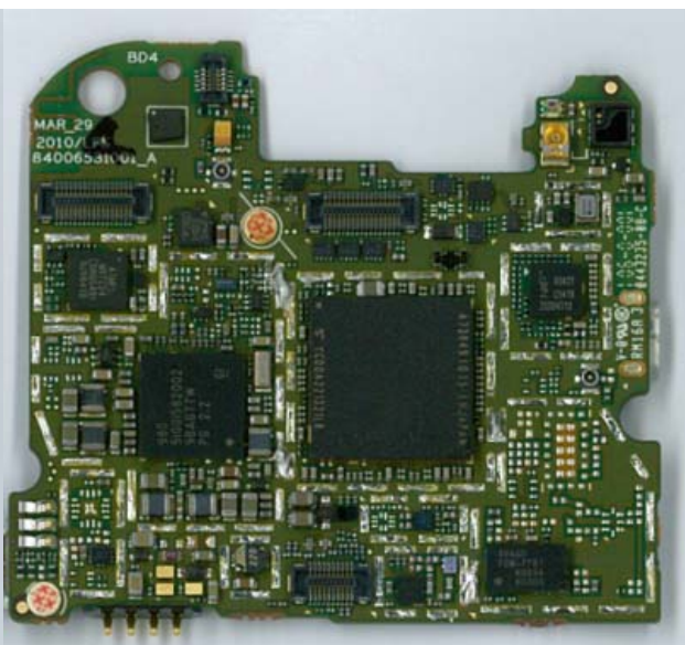
Main Board Bottom W/O shields
