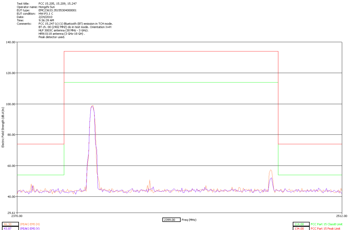
Authorized Band Emissions Low Channel Dual Polarization X
