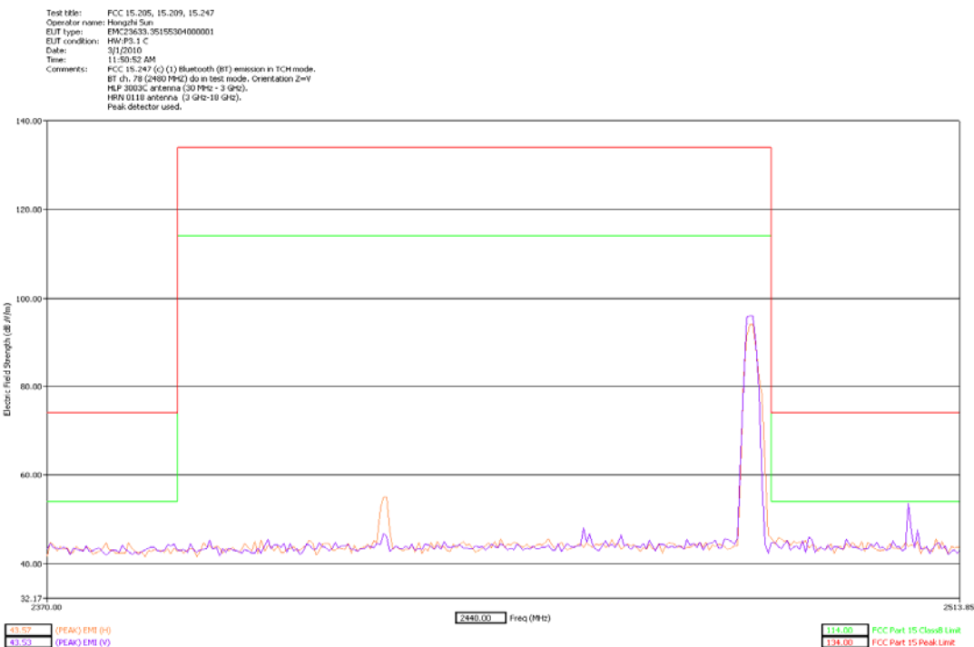
Authorized Band Emissions High Channel Dual Polarization Z
