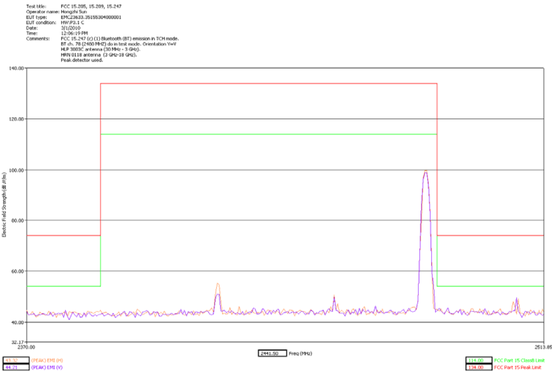
Authorized Band Emissions High Channel Dual Polarization Y
