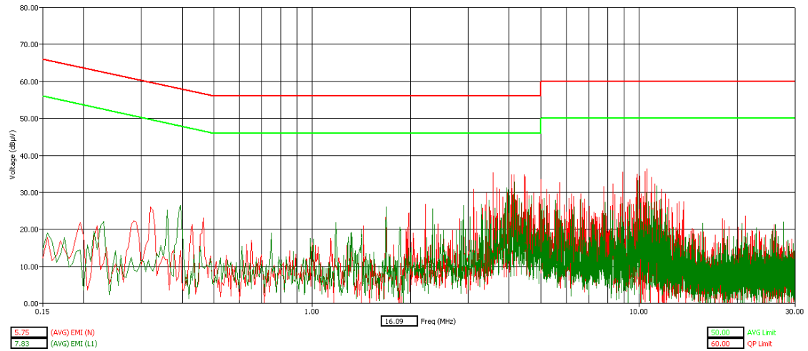
WLAN Channel 1 - Tx Mode - AVG Detector
