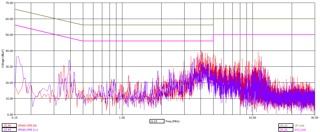
WLAN Channel 6 - Tx Mode - Peak Detector
