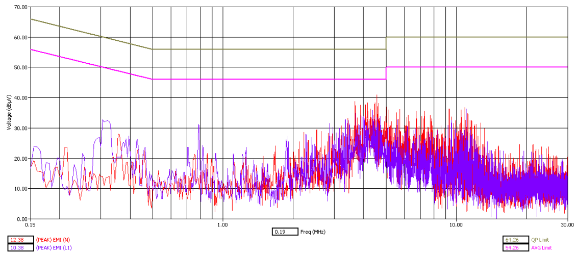
WLAN Channel 6 - Tx Mode - Peak Detector
