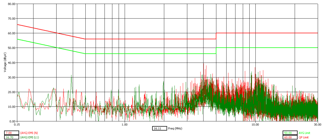
WLAN Channel 11 - Tx Mode - AVG Detector
