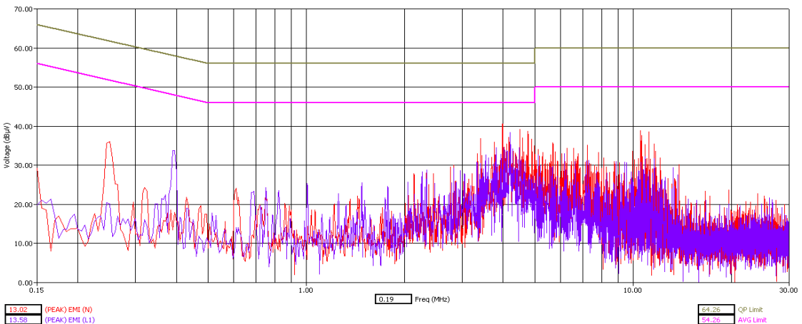
WLAN Channel 11 - Tx Mode - Peak Detector
