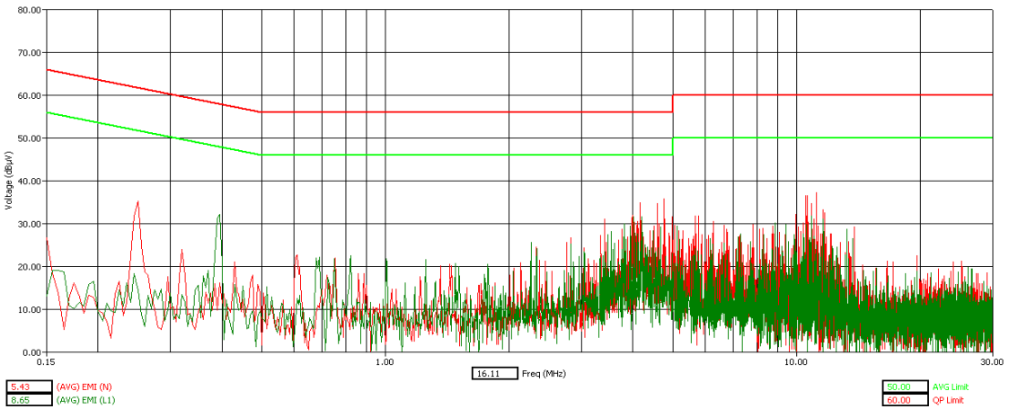
WLAN Channel 11 - Tx Mode - AVG Detector
