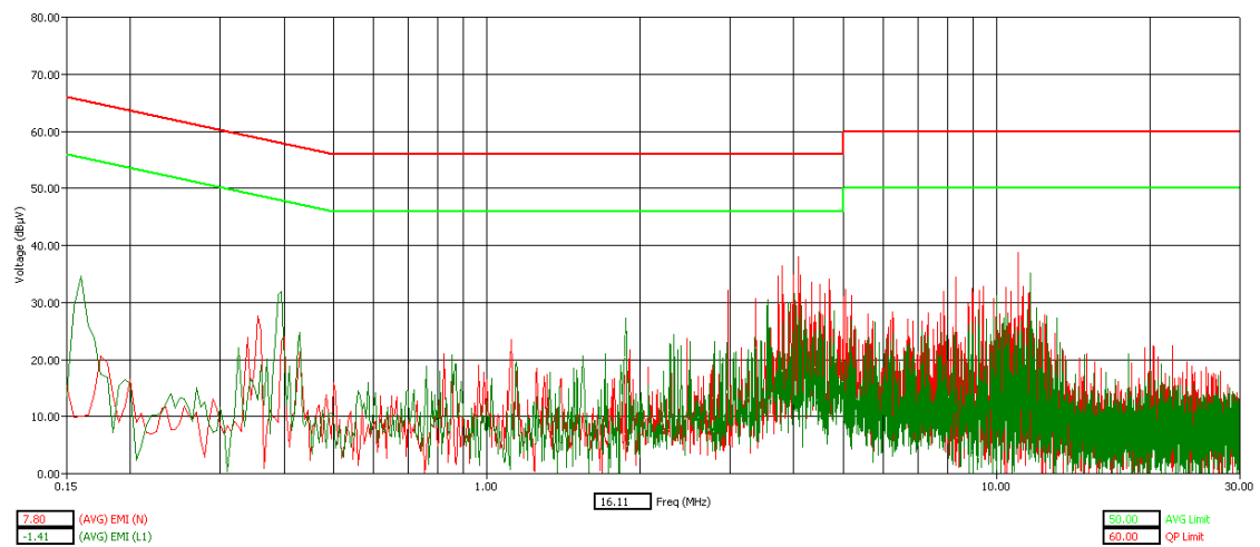
WLAN Channel 6 - Tx Mode - AVG Detector
