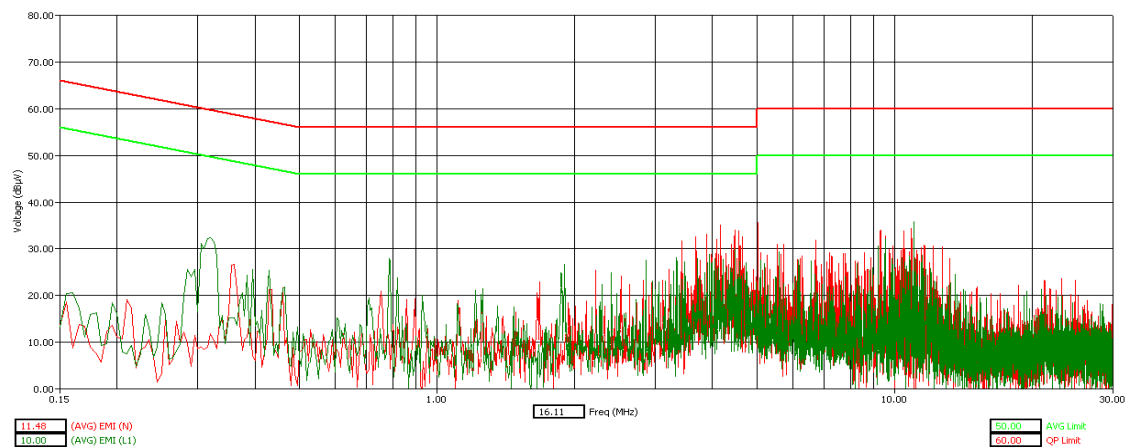
WLAN Channel 6 - Tx Mode - AVG Detector
