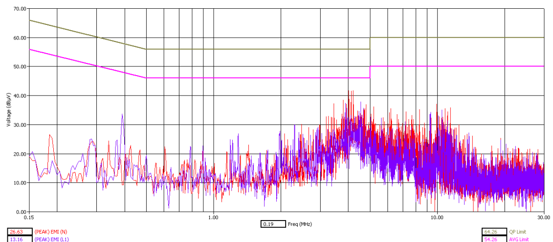
WLAN Channel 11 - Tx Mode - Peak Detector
