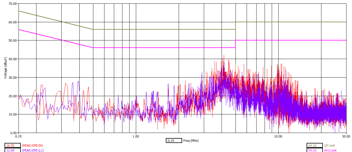
WLAN Channel 1 - Tx Mode - Peak Detector
