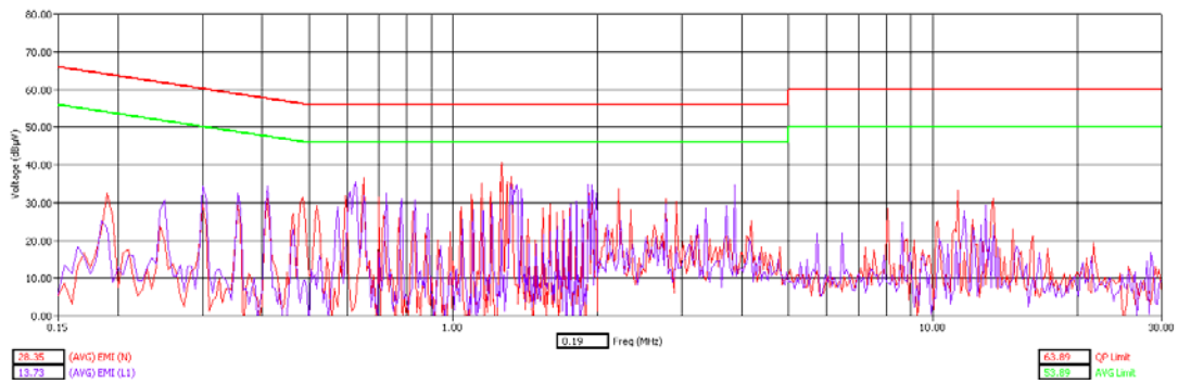
Bluetooth – Hopping - Tx Mode – Average Detector
