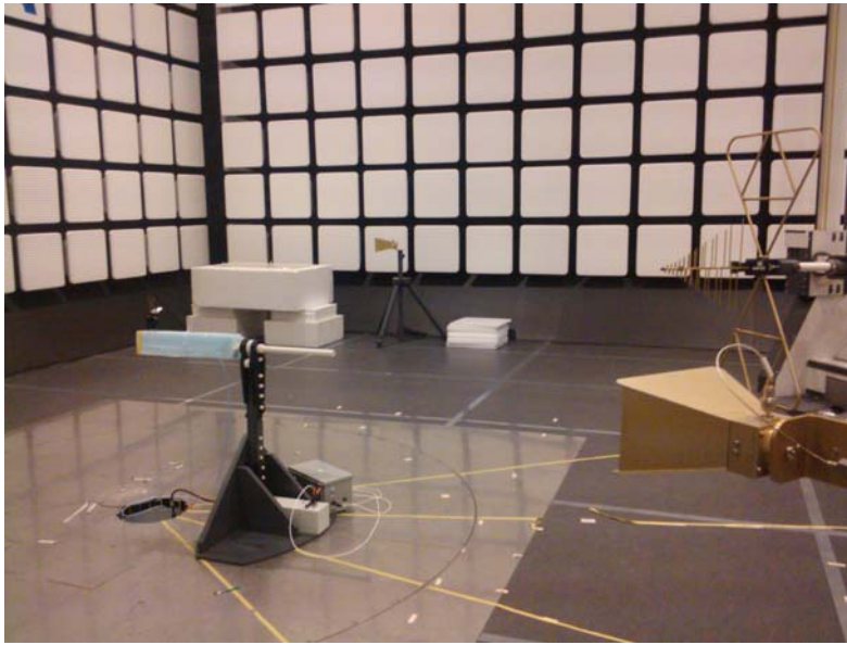
Radiated Emissions
