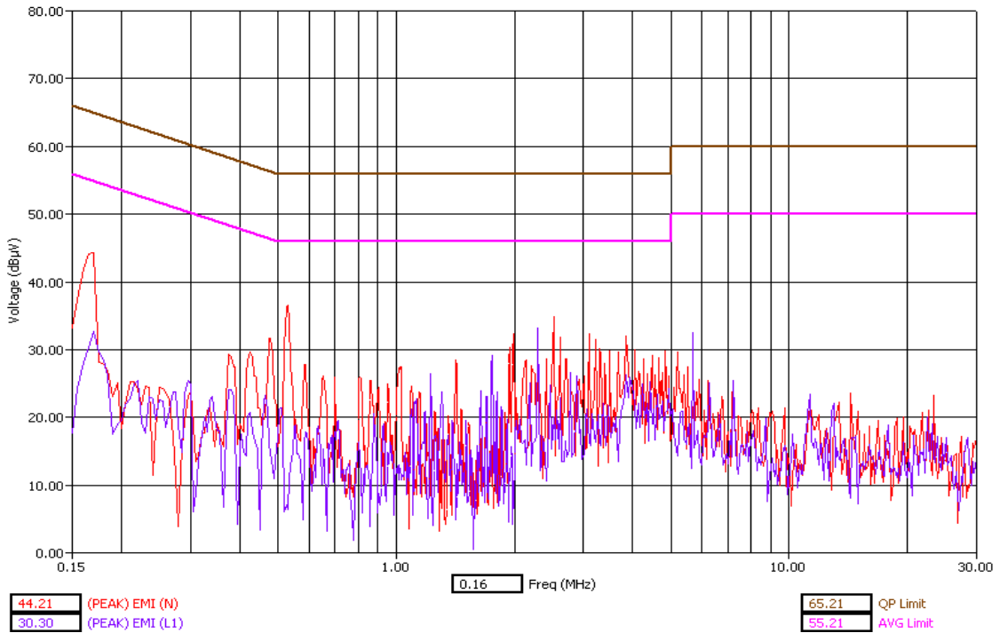
Bluetooth – Hopping - Tx Mode – Peak Detector
