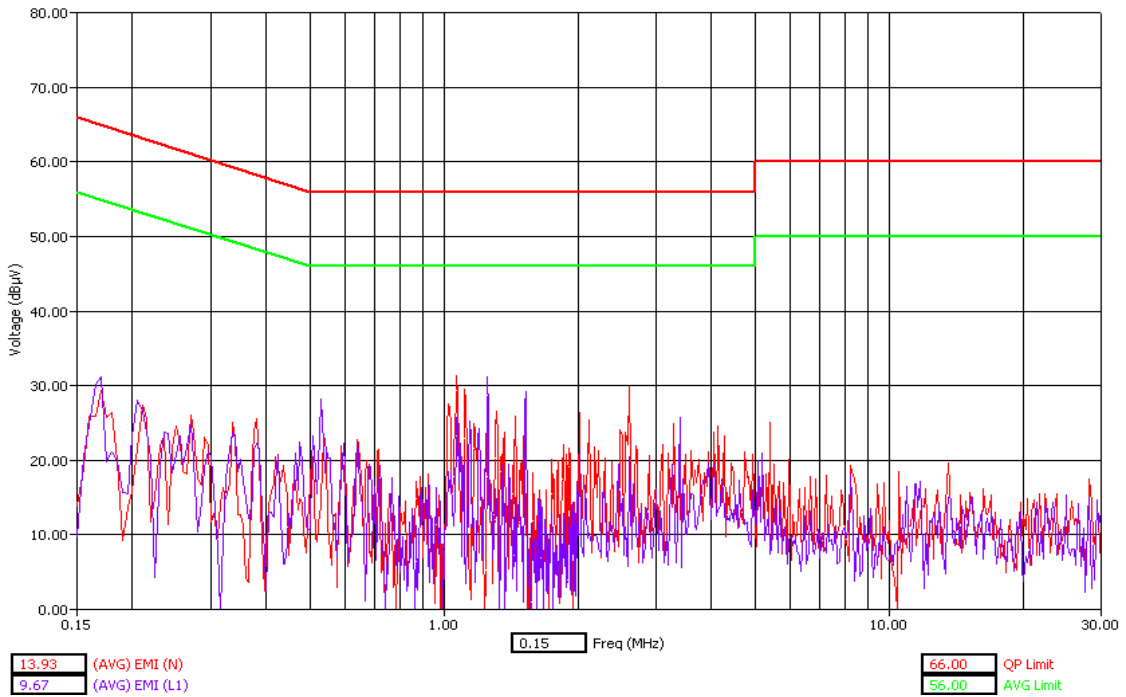
Bluetooth – Hopping - Tx Mode – Average Detector
