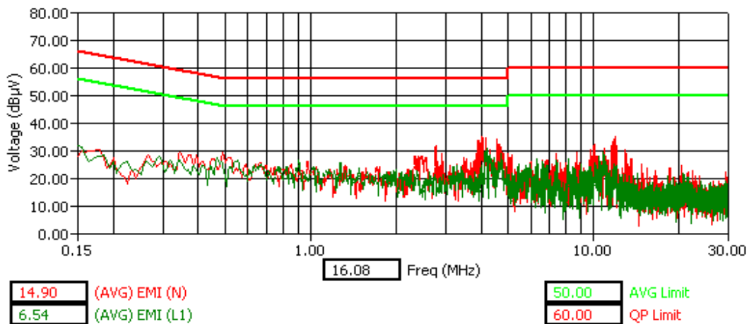
WLAN Channel 6 - Tx Mode - AVG Detector
