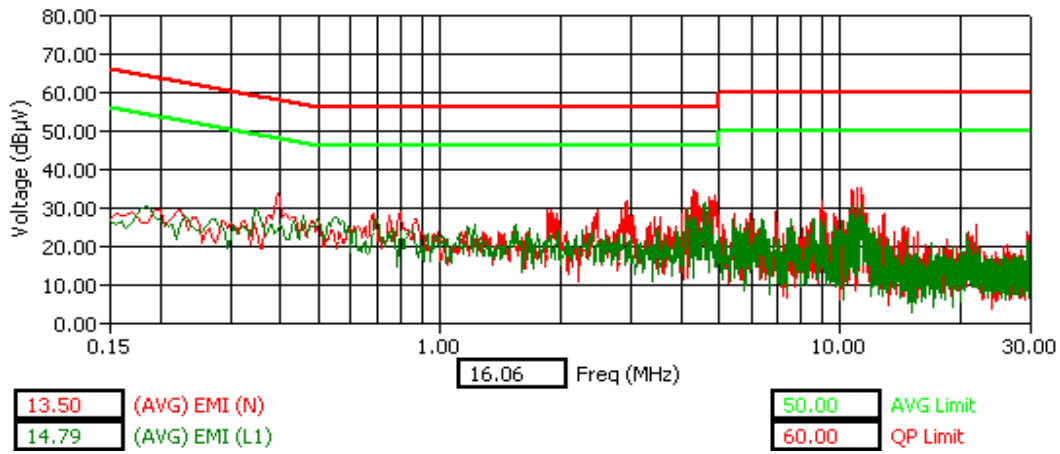
WLAN Channel 11 - Tx Mode - AVG Detector
