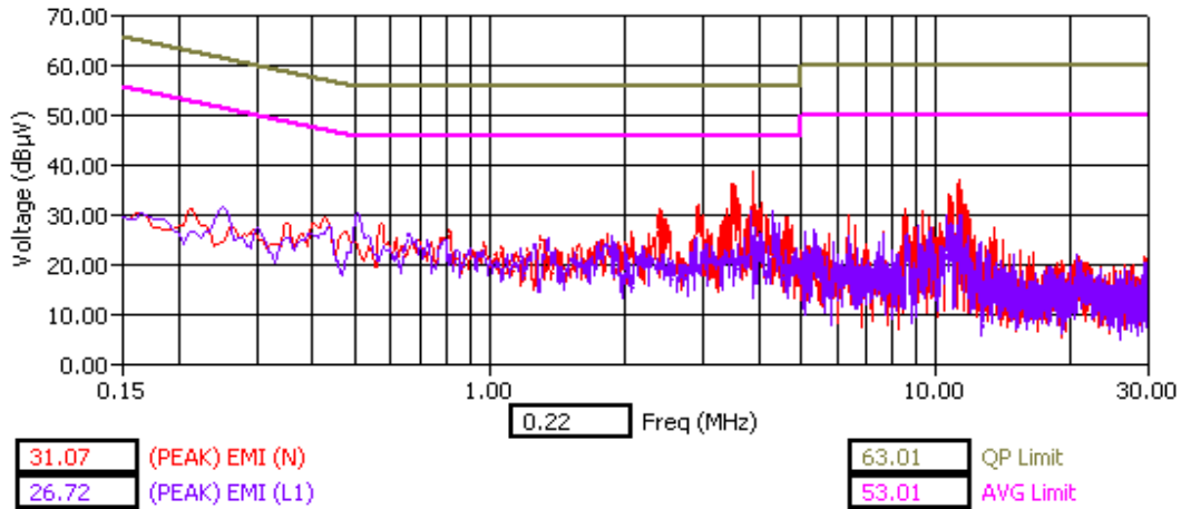
WLAN Channel 6 - Tx Mode - Peak Detector
