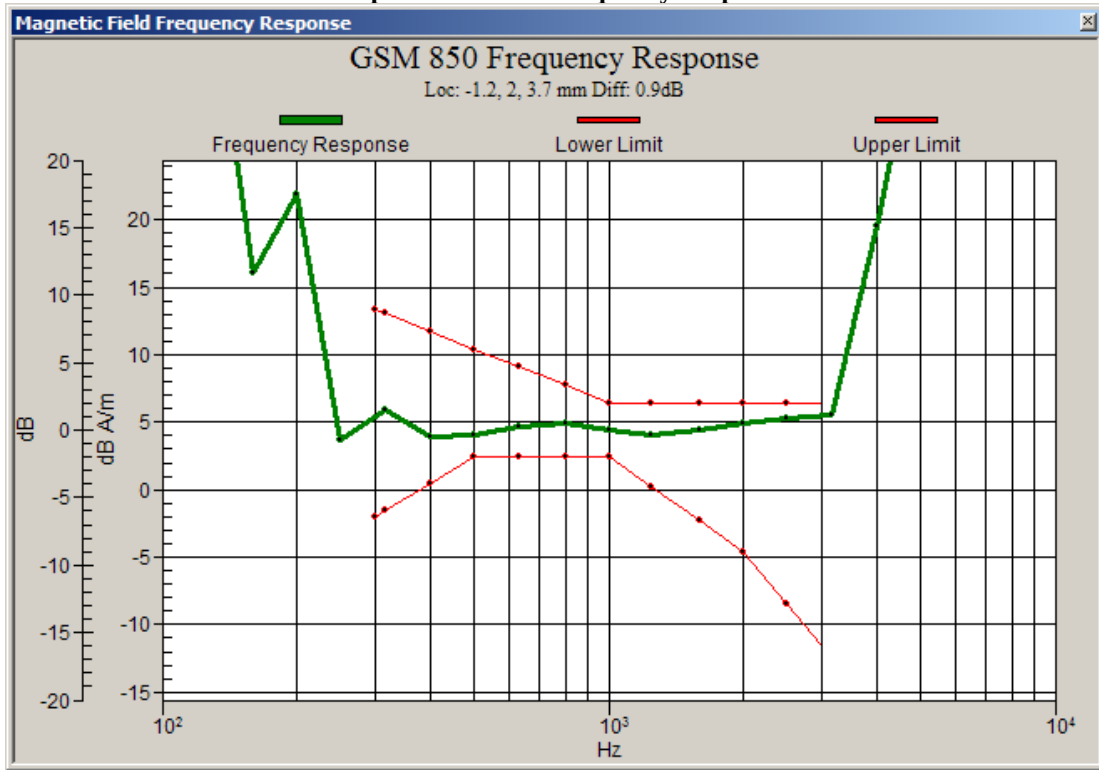
Graph 2: GSM 850 Frequency Response
