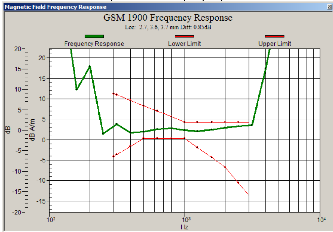
Graph 3: GSM 1900 Frequency Response
