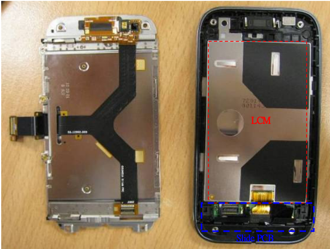
Case B with Slide FPC
