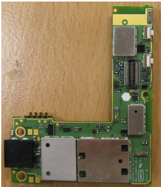
Main Board Top With Shields
