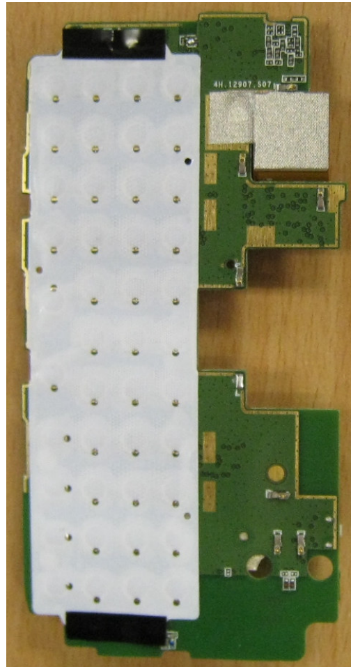
Keypad Board Bottom
