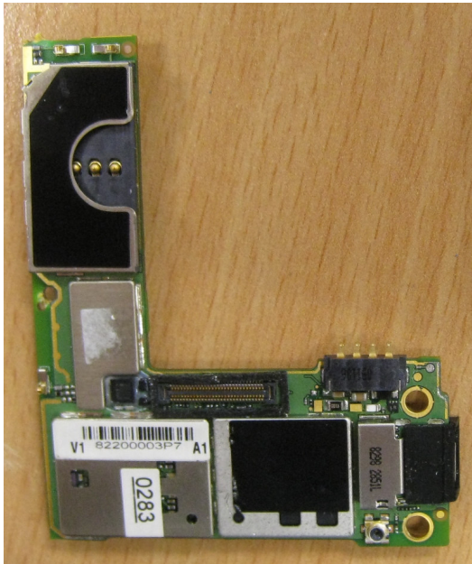
Main Board Bottom With Shields
