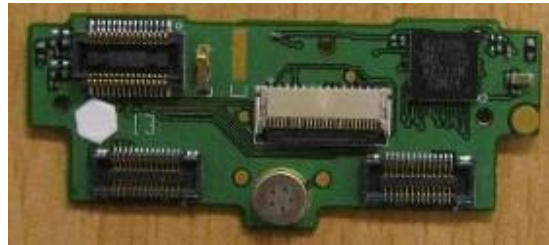
Bottom of Slide PCB
