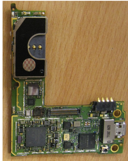
Main Board Bottom Without Shields
