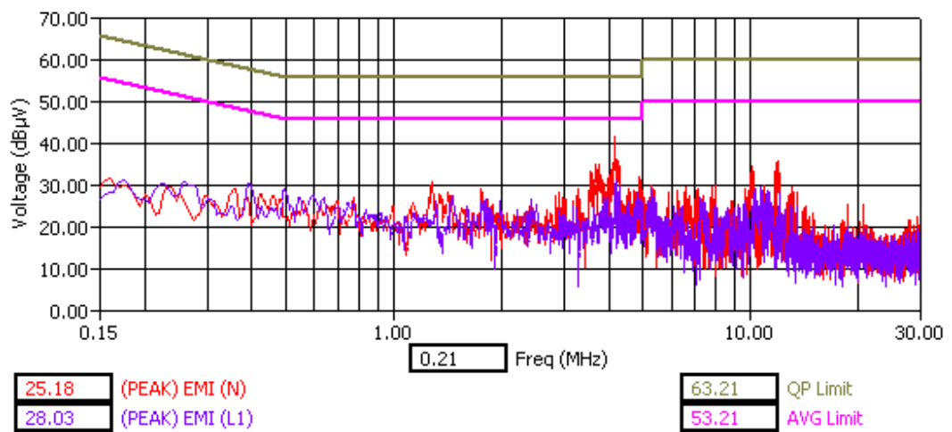
WLAN Channel 11 - Tx Mode - Peak Detector
