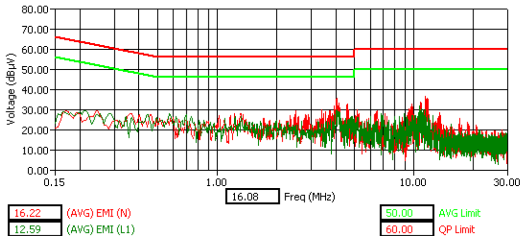
WLAN Channel 6 - Tx Mode - AVG Detector
