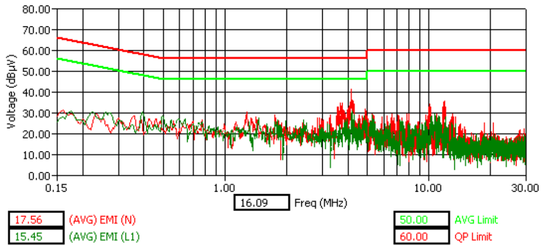
WLAN Channel 11 - Tx Mode - AVG Detector
