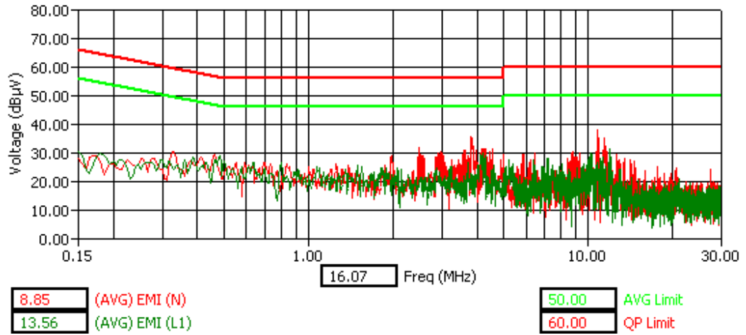
WLAN Channel 1 - Tx Mode - AVG Detector
