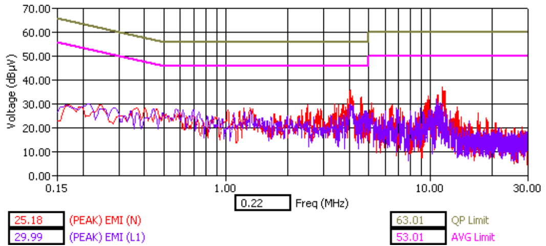
WLAN Channel 6 - Tx Mode - Peak Detector
