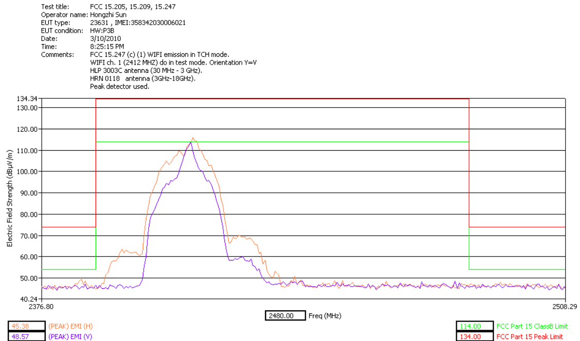
Low Band Edge Y Orientation – slider open
