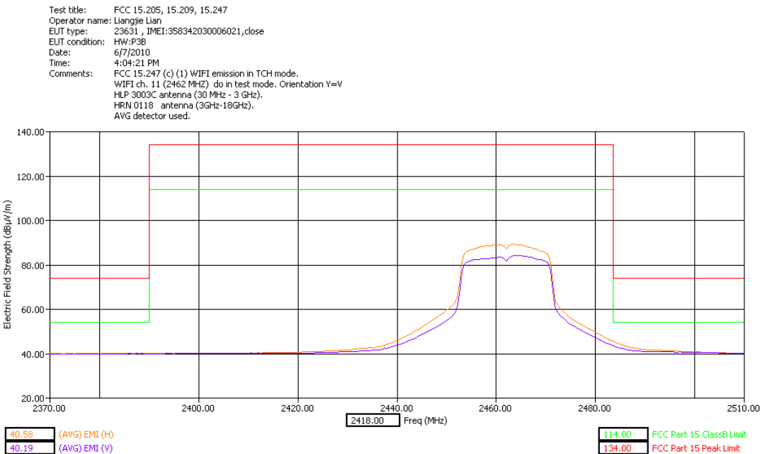
High Band Edge Y Orientation – slider closed
