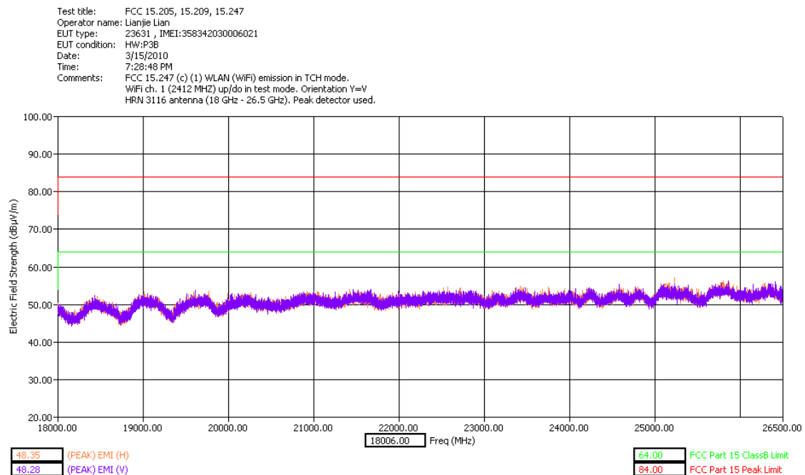
18 – 26.5 GHz Low Channel Dual Polarization Y- slider closed
