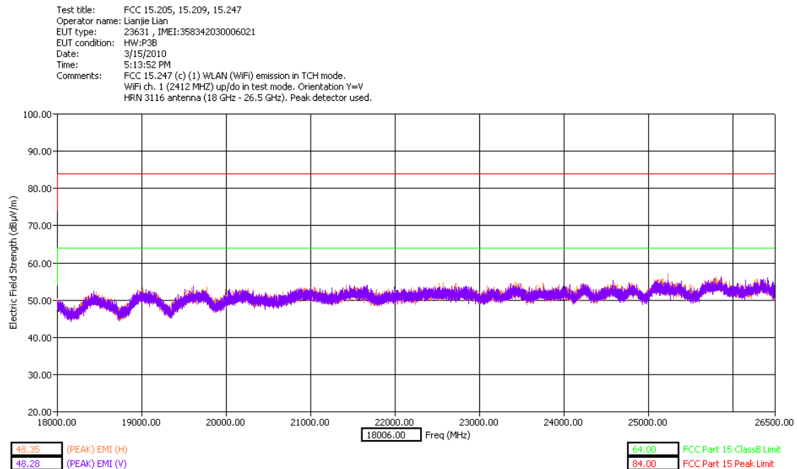
18 – 26.5 GHz Low Channel Dual Polarization Y- slider open
