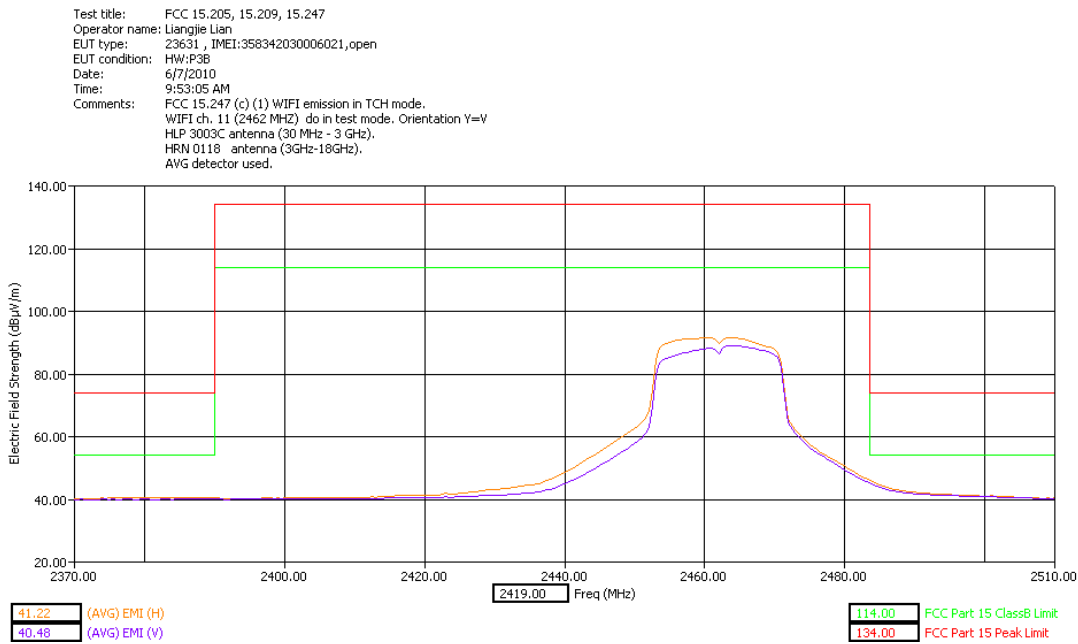
High Band Edge Y Orientation – slider open
