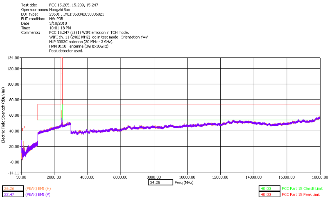
30 - 18000MHz High Channel Dual Polarization Y - slider open
