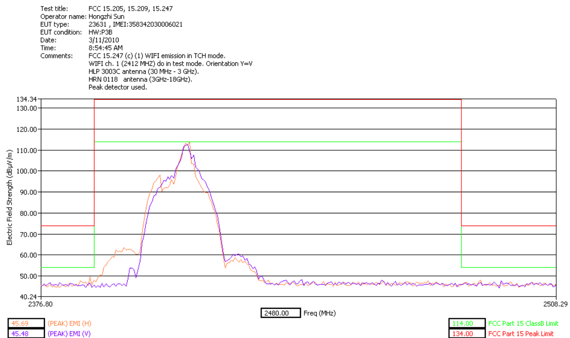
Low Band Edge Y Orientation – slider closed
