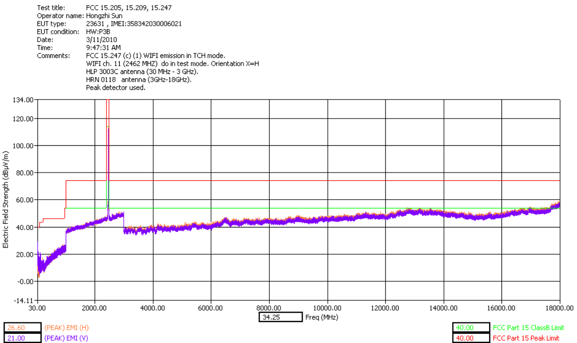
30 - 18000MHz High Channel Dual Polarization X - slider closed
