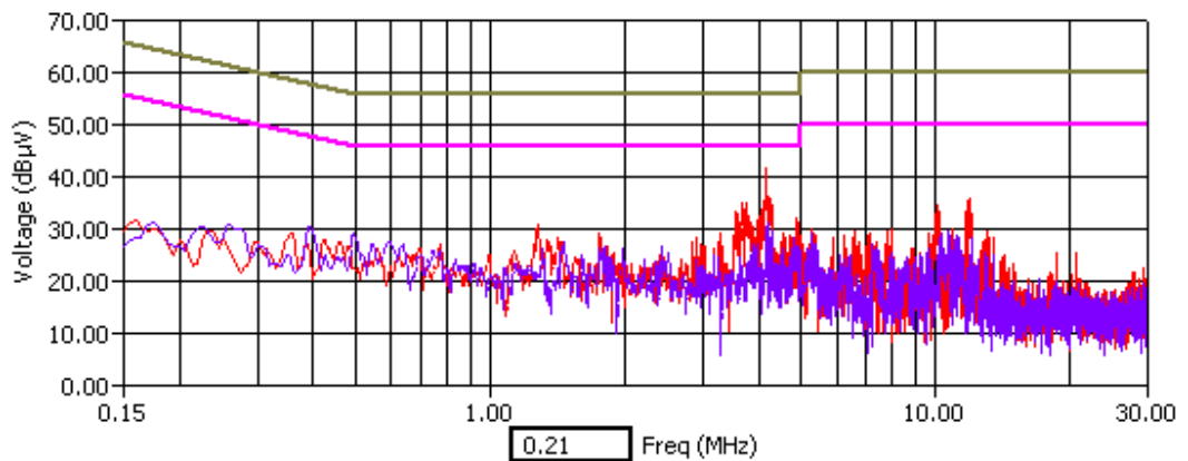
WLAN Channel 11 - Tx Mode - Peak Detector
