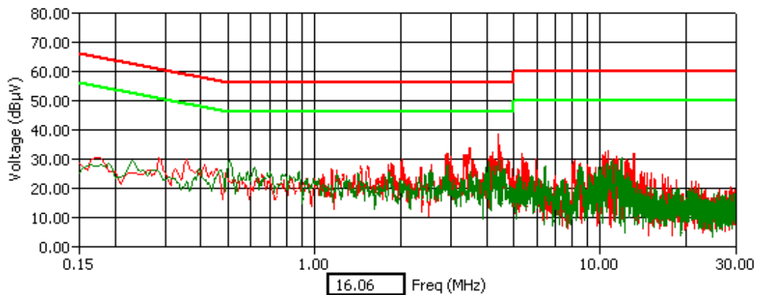
WLAN Channel 6 - Tx Mode - AVG Detector
