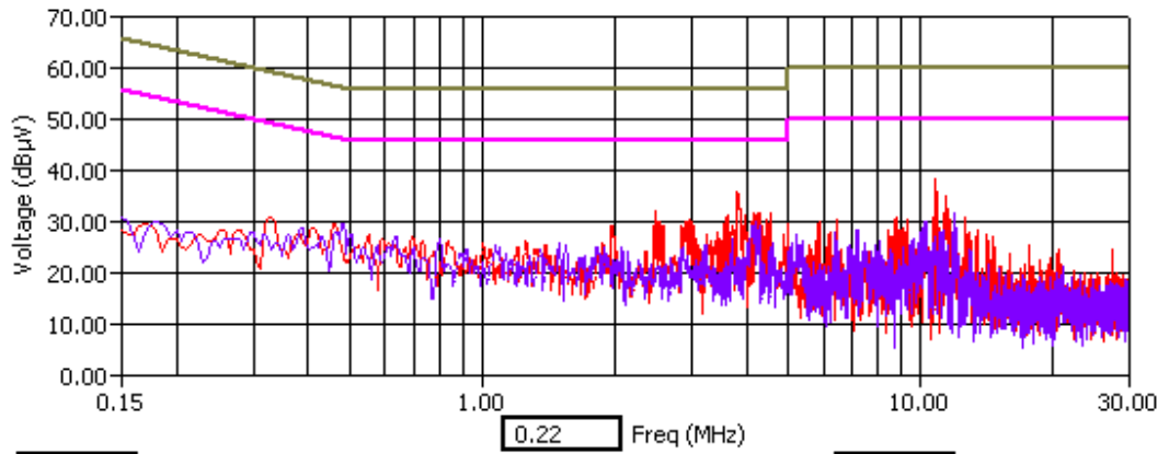
WLAN Channel 1 - Tx Mode - Peak Detector
