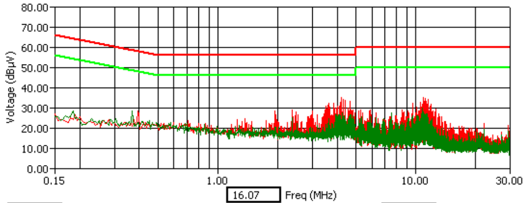
WLAN Channel 1 - Tx Mode - AVG Detector
