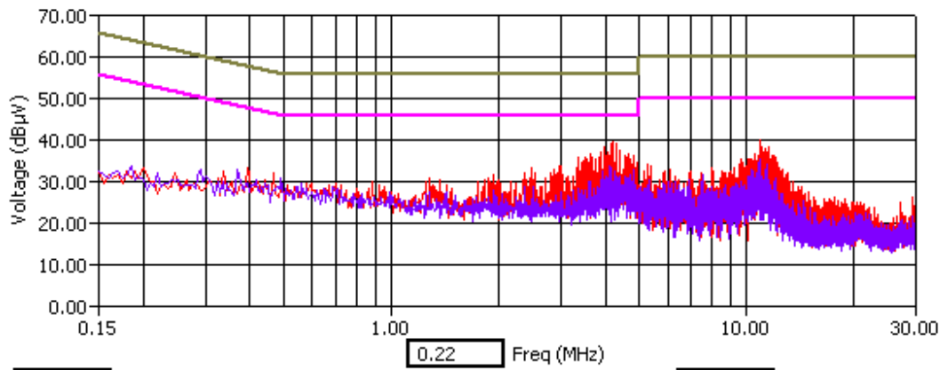
WLAN Channel 1 - Tx Mode - Peak Detector
