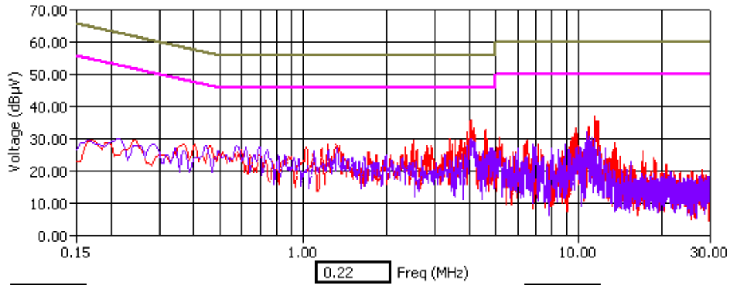
WLAN Channel 6 - Tx Mode - Peak Detector
