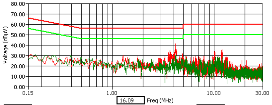
WLAN Channel 11 - Tx Mode - AVG Detector
