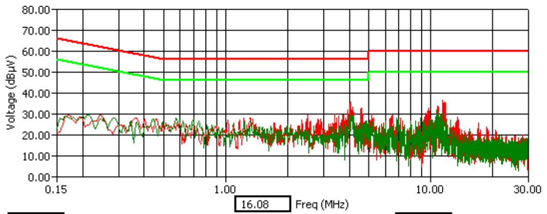
WLAN Channel 6 - Tx Mode - AVG Detector
