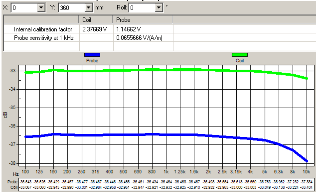
Graph 1: Frequency Response measured in AMCC
