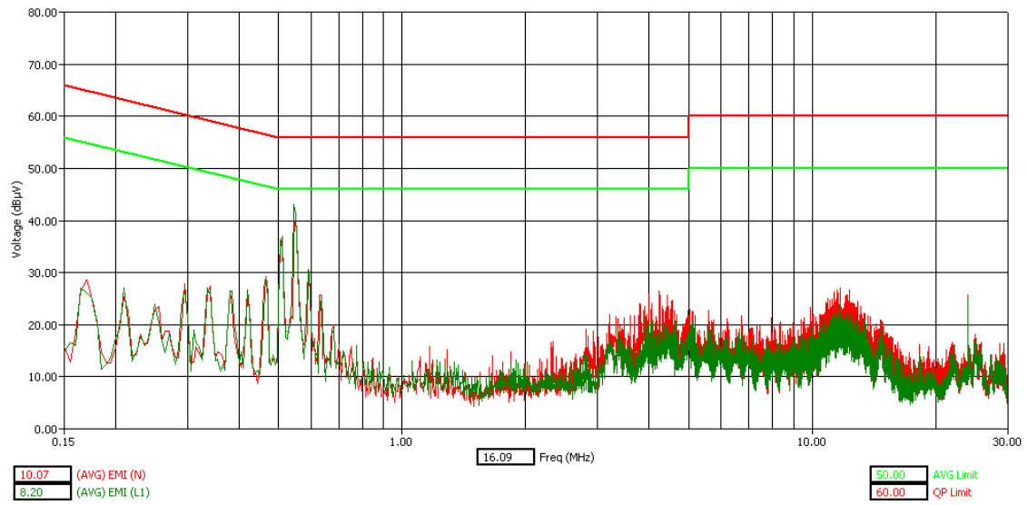
Bluetooth - Hopping - Tx Mode - AVG Detector
