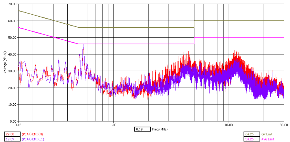
Bluetooth - Hopping - Tx Mode - Peak Detector
