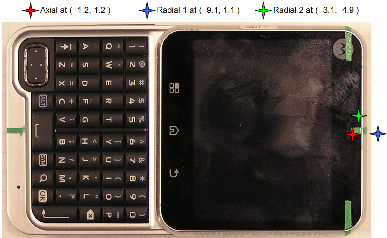
Figure 5. Location of point measurements for ABM (Telecoil) Emissions
