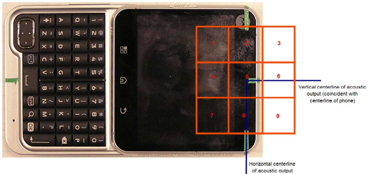
Figure 2. Phone Front - Orientation and Measurement Plane for RF Emissions Testing
