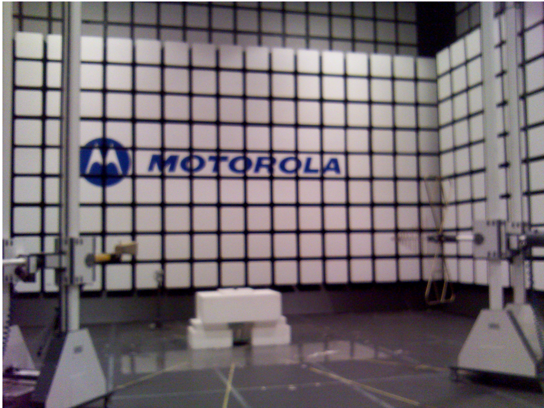
RE Setup for BT radiated test
