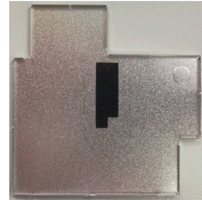
Shield-cover Back view
