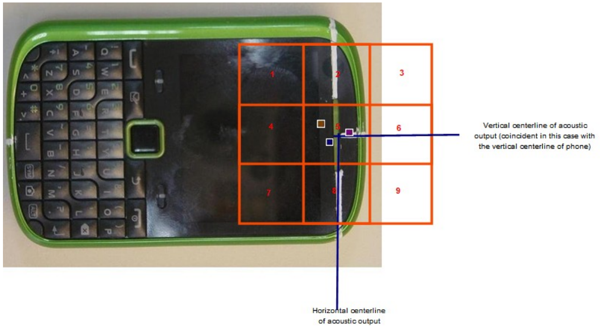
Figure 3. Phone Open - Orientation and Measurement Plane for RF Emissions Testing
