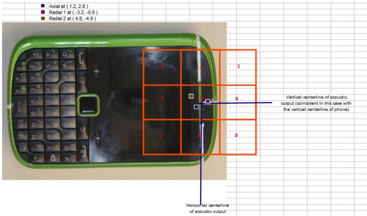
Figure 6. Location of Measured Points for T-coil measurements
