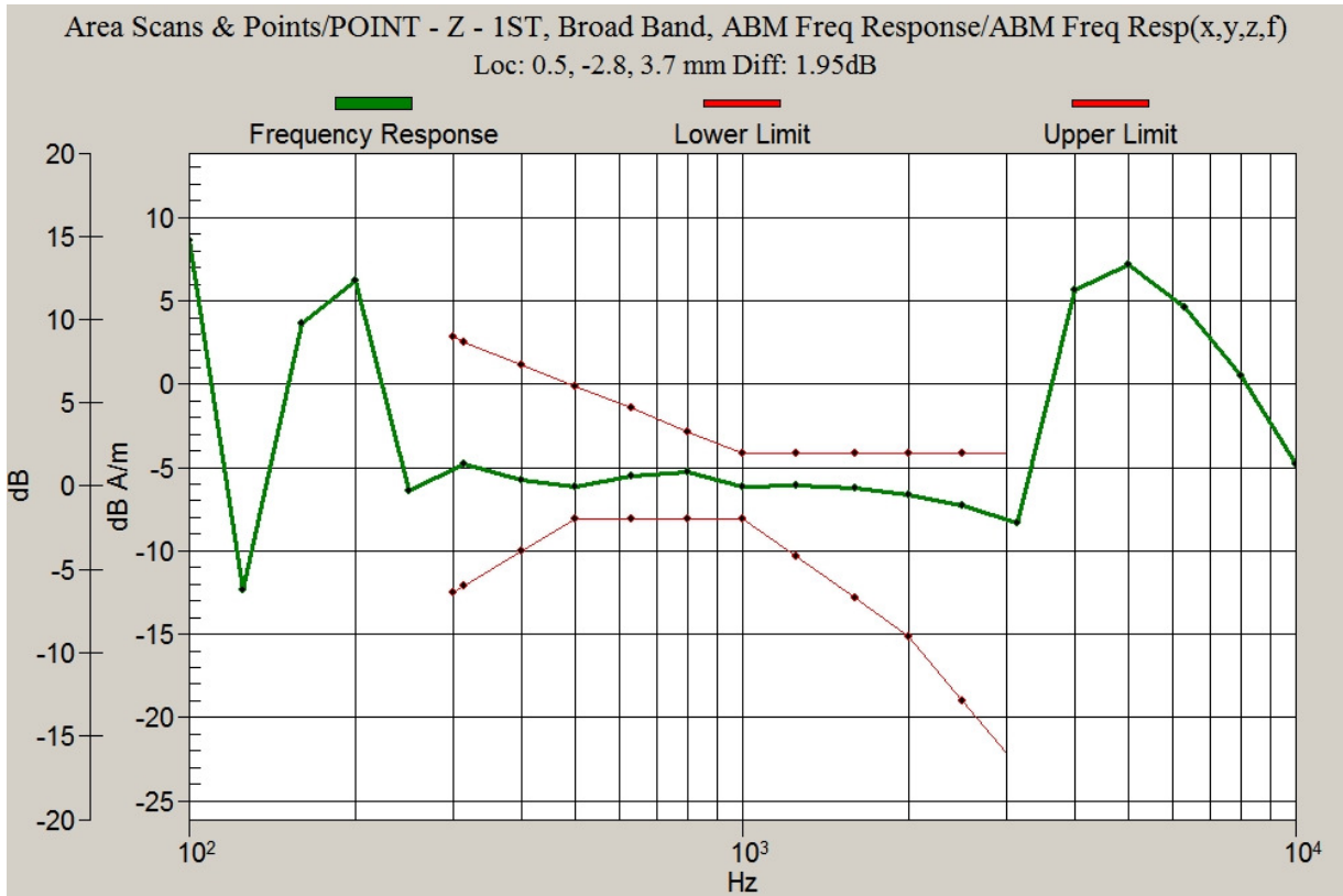
Graph 10: CDMA 1900 Frequency Response
