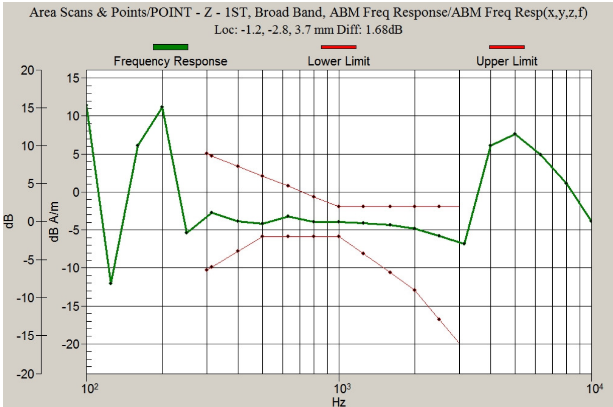
Graph 6: CDMA 1700 Frequency Response
