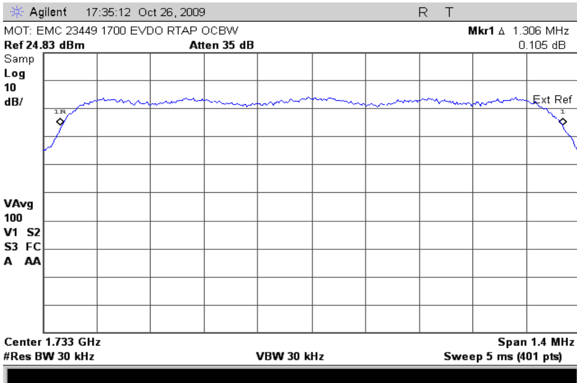
EV-DO 1700 – Channel 4500 (1732.50 MHz) – Occupied Bandwidth
