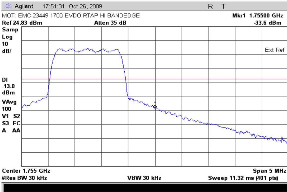
EV-DO 1700 – Upper Band Edge – Channel 875 (1753.75 MHz)
