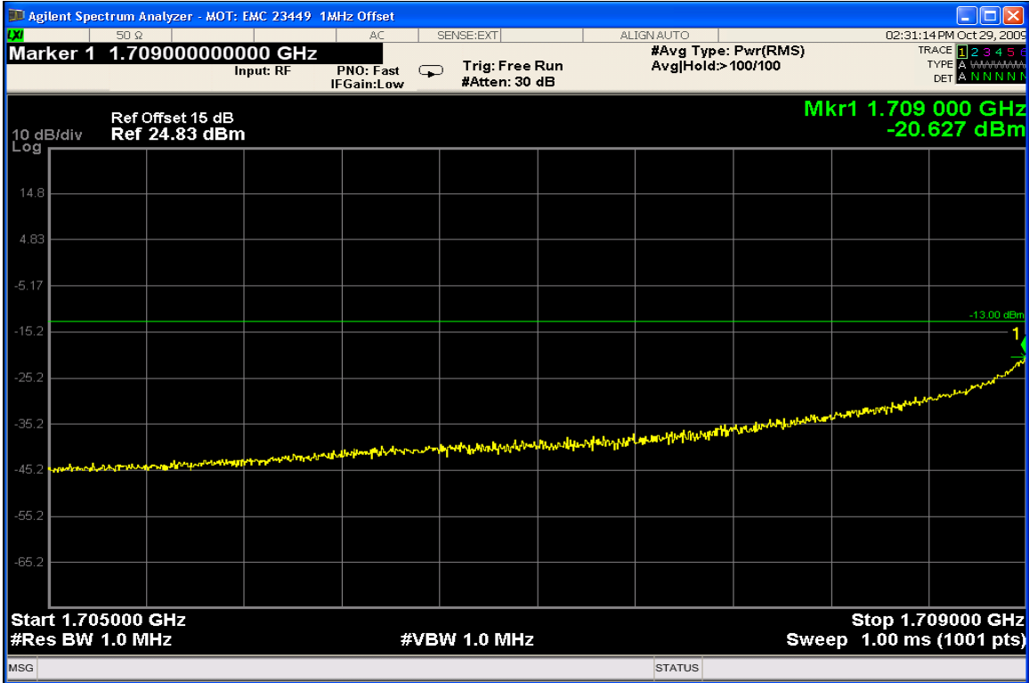
AWS Conducted Spurious Emissions (Lower adjacent 1 MHz band)
