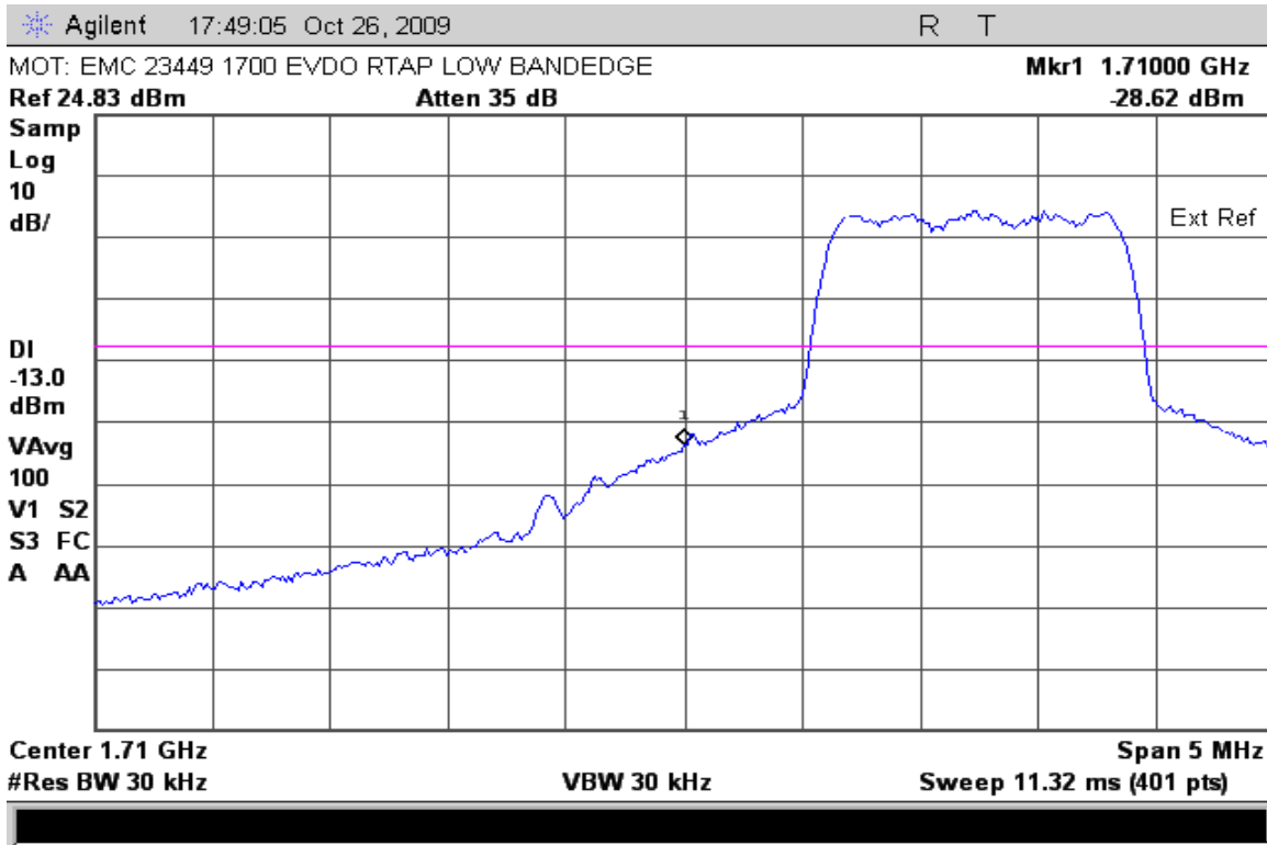
EV-DO 1700 – Lower Band Edge – Channel 25 (1711.25 MHz)
