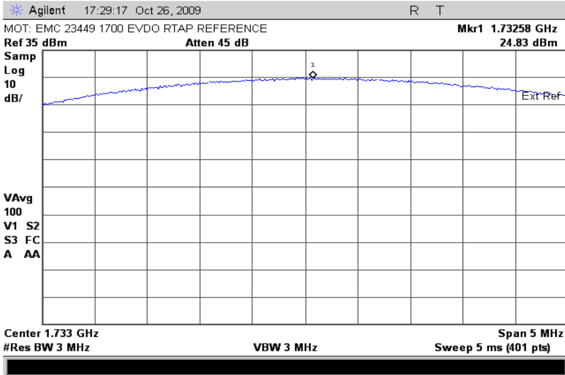
EV-DO 1700 – Reference Level Plot – Channel 450 (1732.50 MHz)
