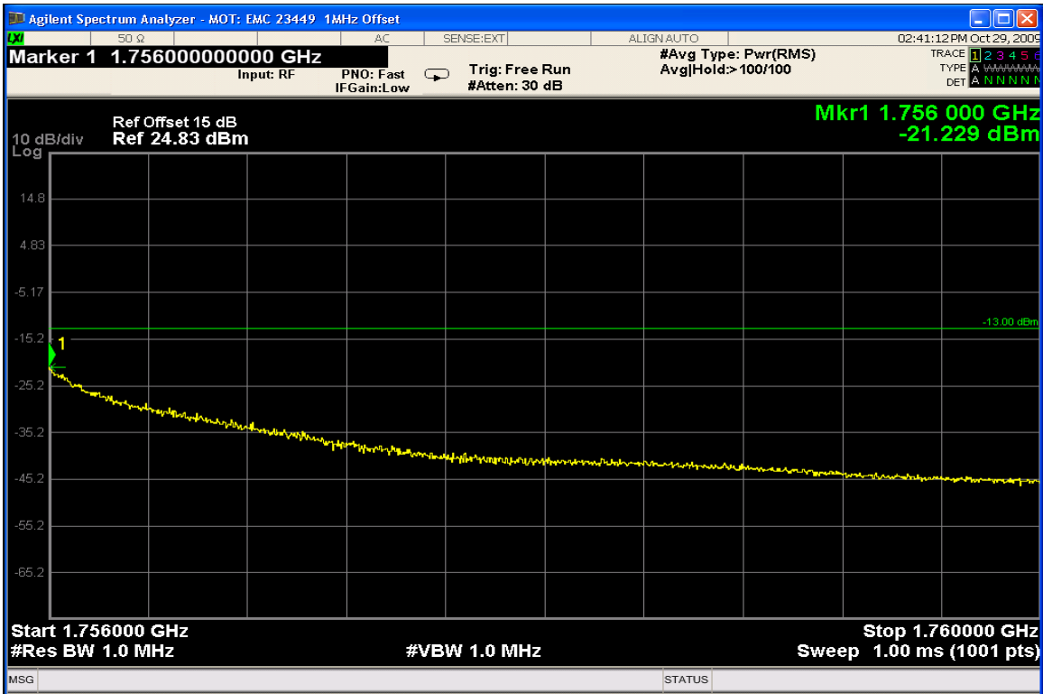
AWS Conducted Spurious Emissions (Upper adjacent 1 MHz band)
