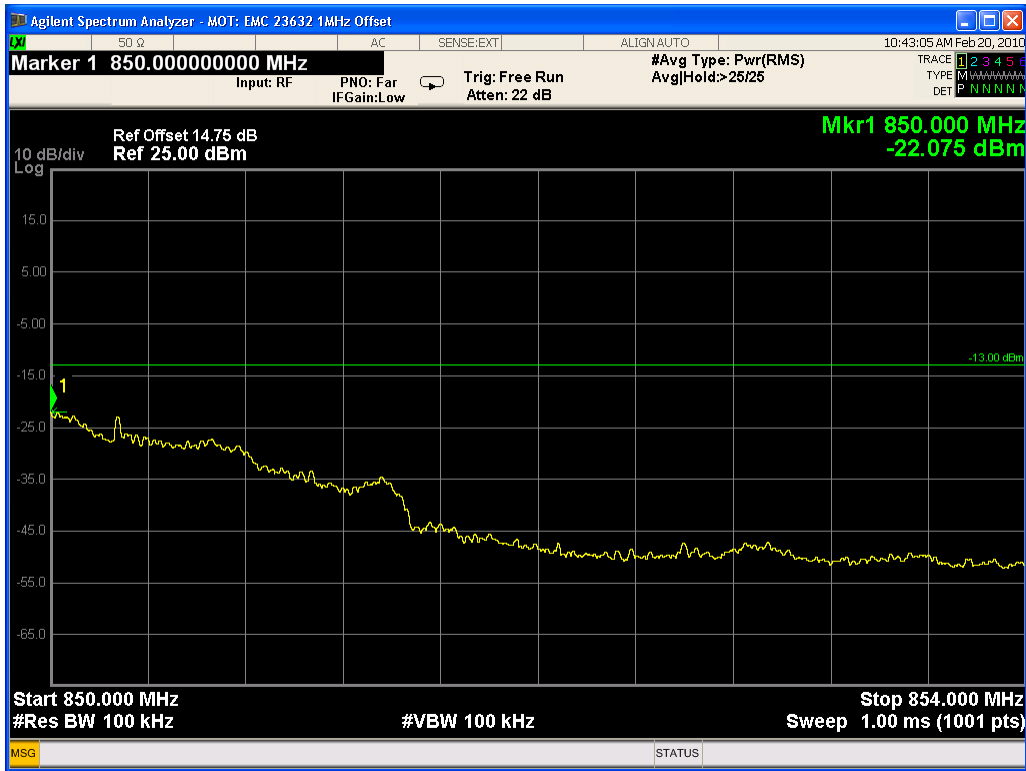
Cellular Conducted Spurious Emissions (Upper adjacent 1 MHz band)
