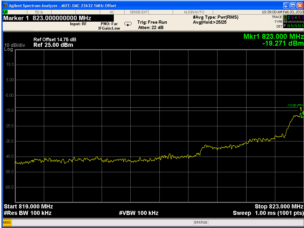
Cellular Conducted Spurious Emissions (Lower adjacent 1 MHz band)
