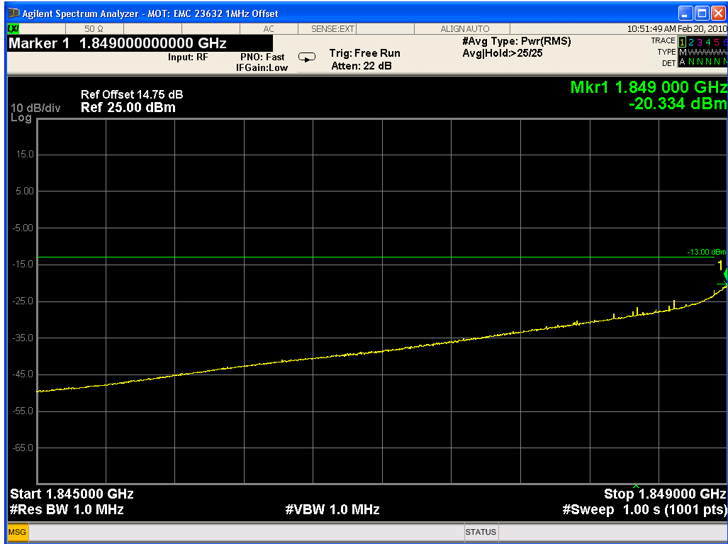
PCS Conducted Spurious Emissions (Lower adjacent 1 MHz band)
