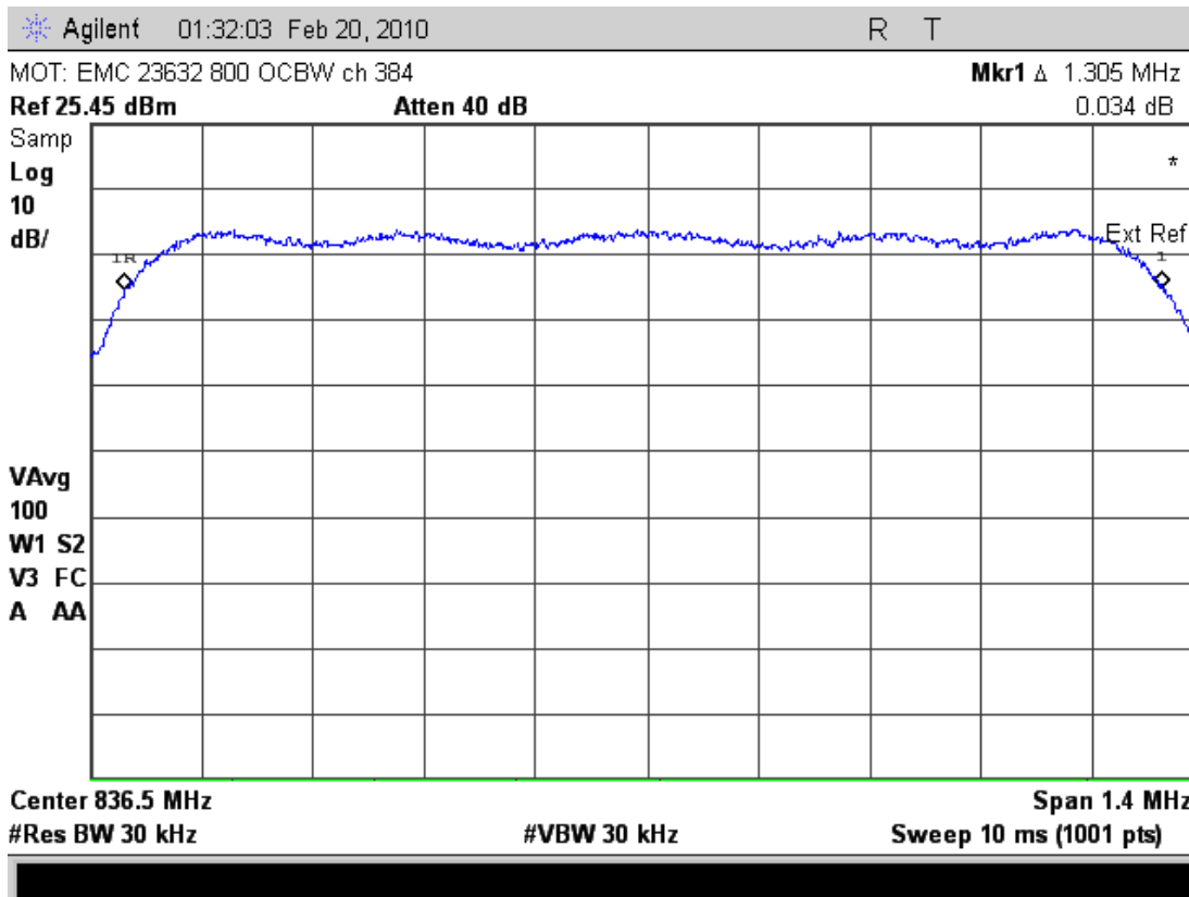
CDMA 800 – Occupied Bandwidth – Channel 384 (836.52MHz)
