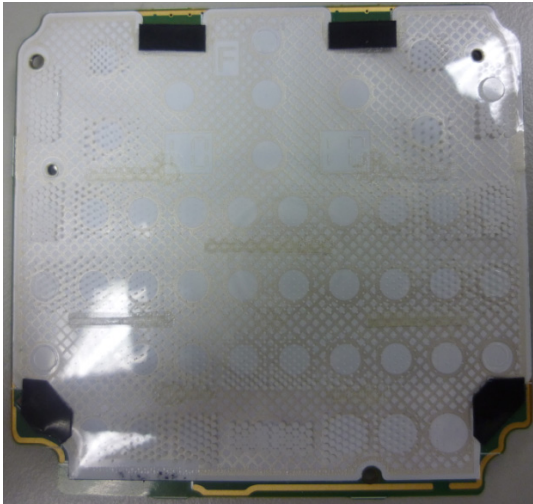
MMI Board Top With Popples
