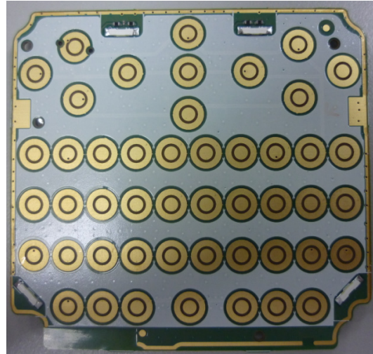
MMI Board Top Without Popples
