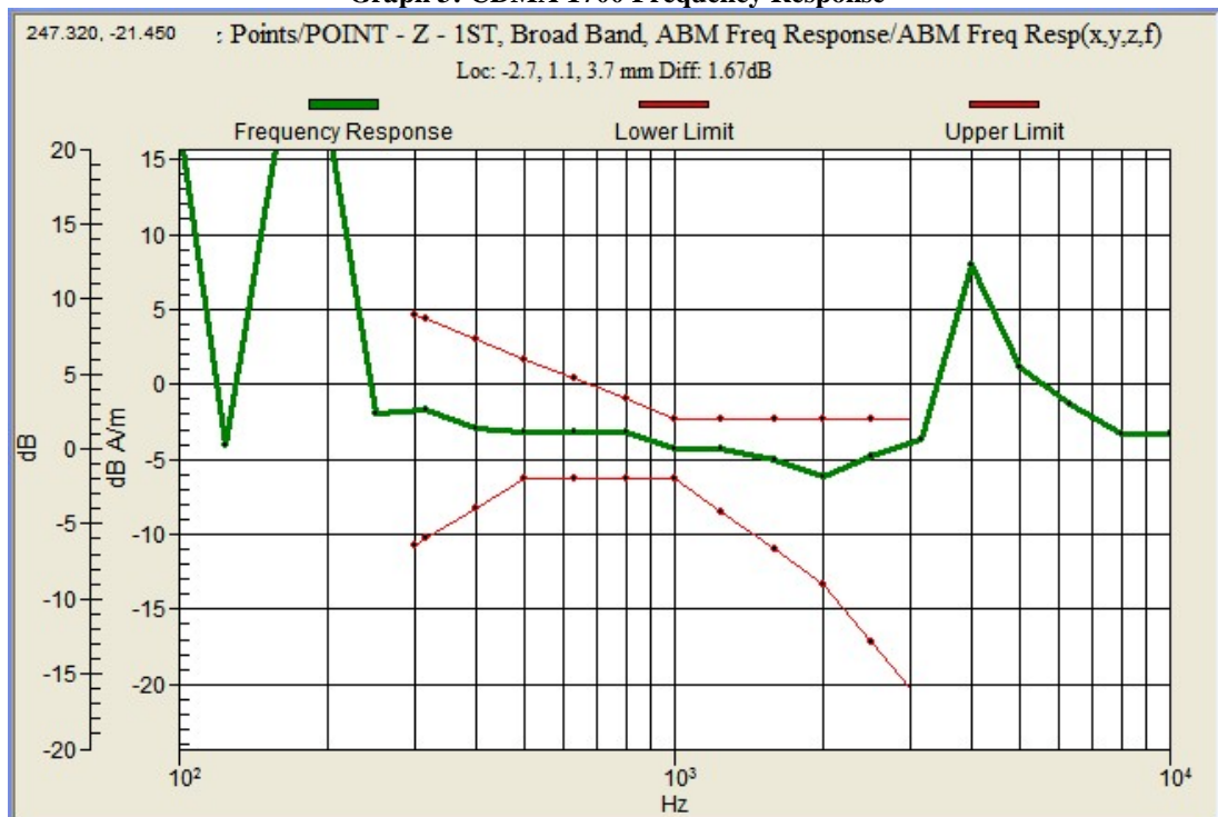
Graph 3: CDMA 1700 Frequency Response
