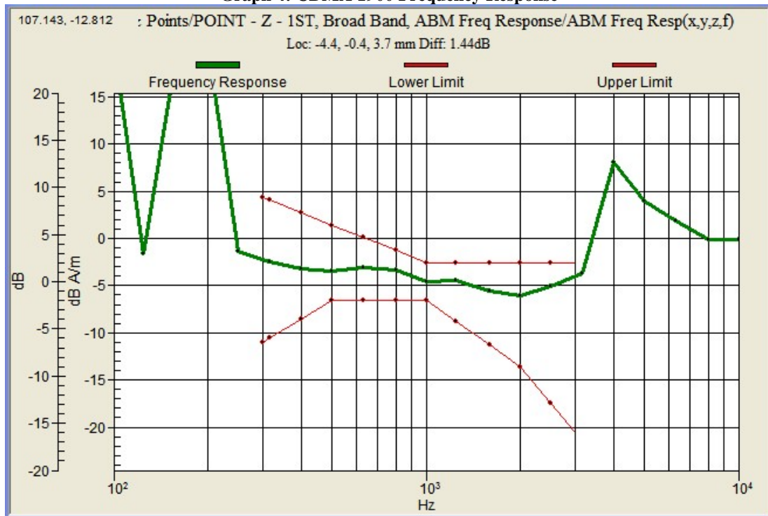
Graph 4: CDMA 1900 Frequency Response
