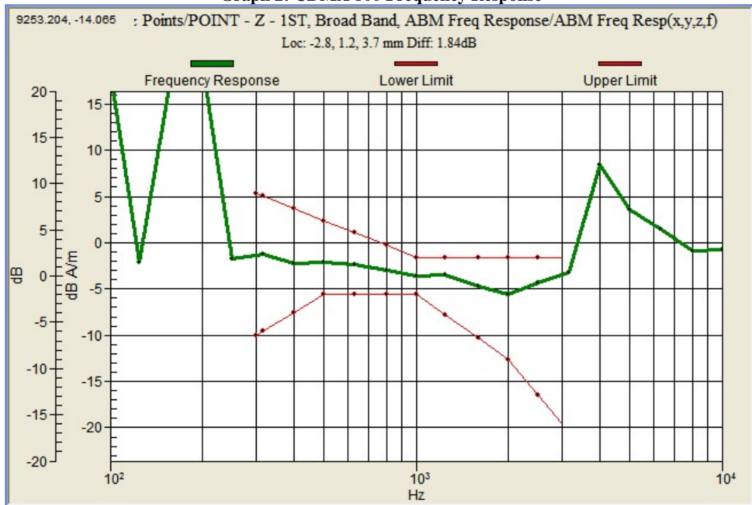
Graph 2: CDMA 800 Frequency Response
