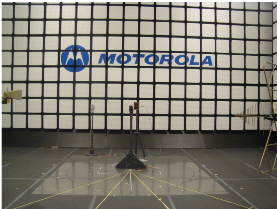
22946-1, IHDT56KY1 setup in semi-anechoic chamber – front view (30 MHz – 18 GHz)
