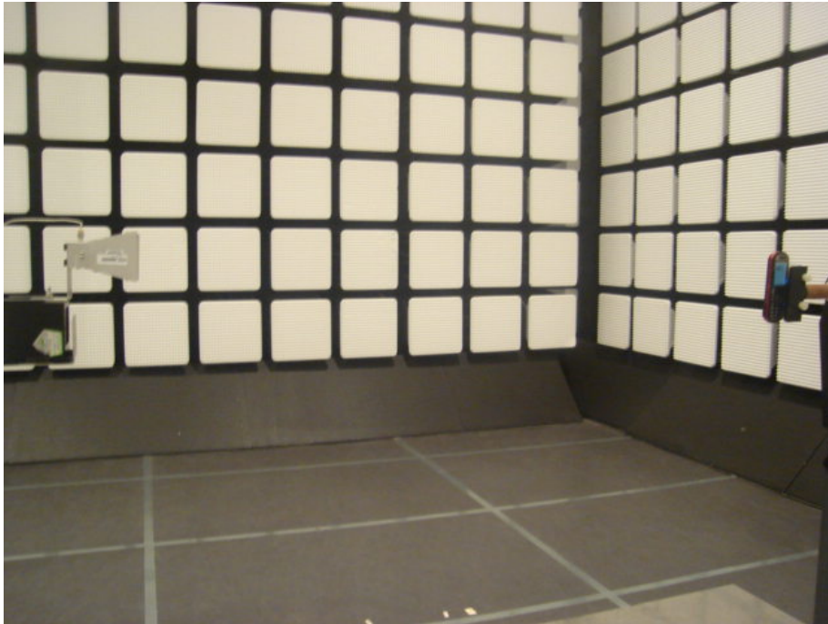
22946-1, IHDT56KY1 setup in semi-anechoic chamber – right view (18 GHz – 26.5 GHz)
