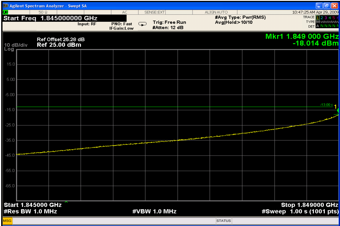
CDMA1900 Ch.25 Lower Band Edge
