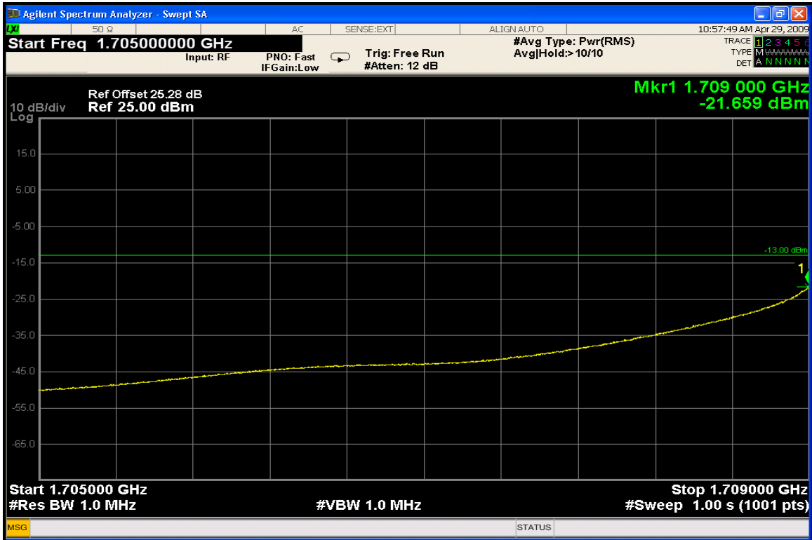
CDMA1700 Ch.25 Lower Band Edge
