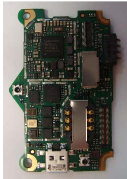
Main Board bottom front Without Shields
