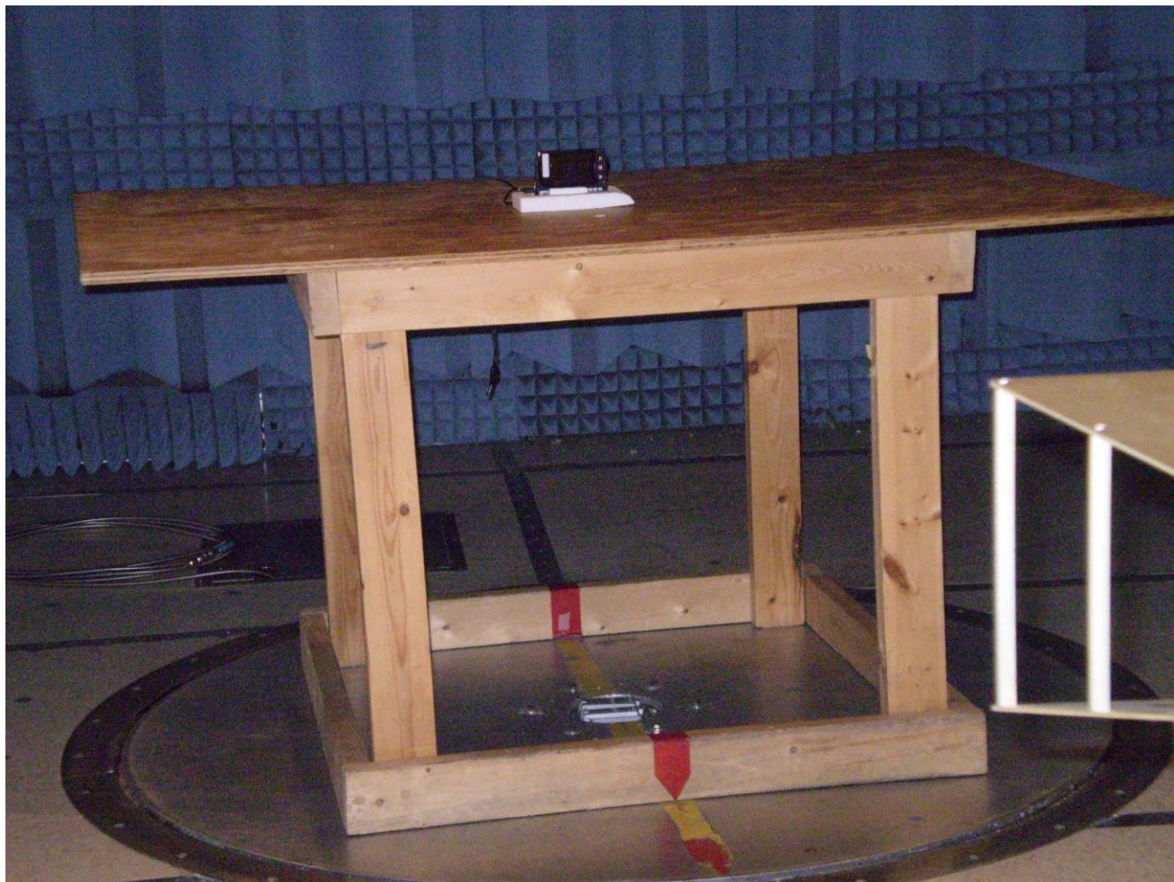
Radiated Emissions
