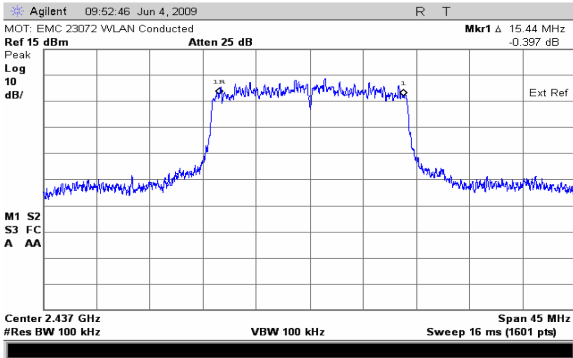
6dB Bandwidth Channel 6 @ 54 Mbps
