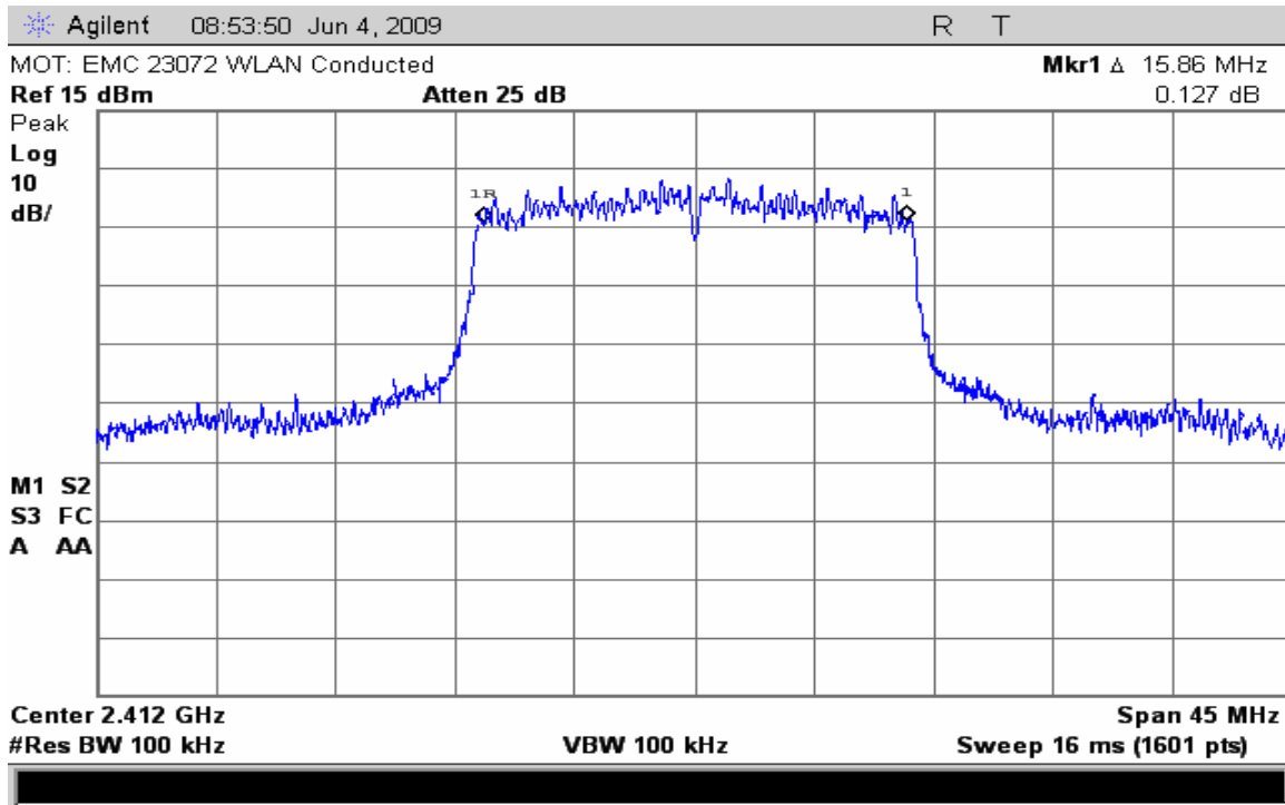
6dB Bandwidth Channel 1 @ 54 Mbps
