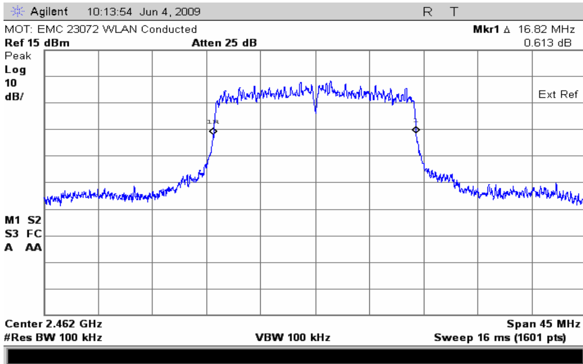
20dB Bandwidth Channel 11 @ 54 Mbps
