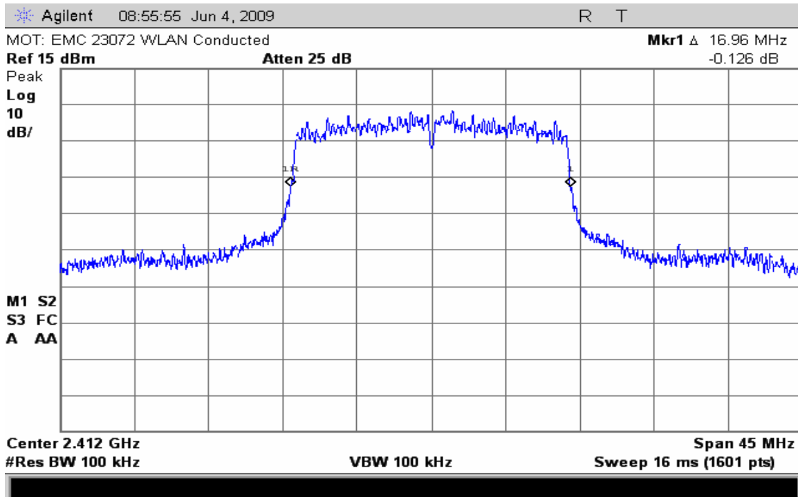
20dB Bandwidth Channel 1 @ 54 Mbps
