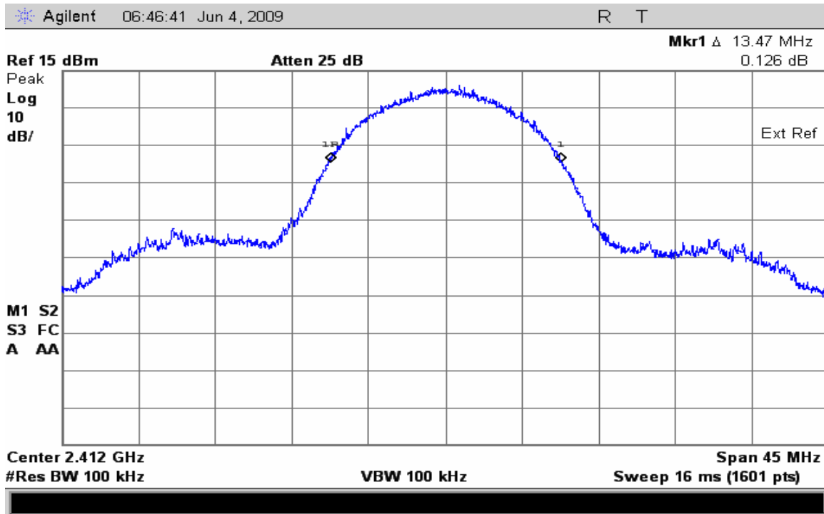
20dB Bandwidth Channel 1 @ 11 Mbps
