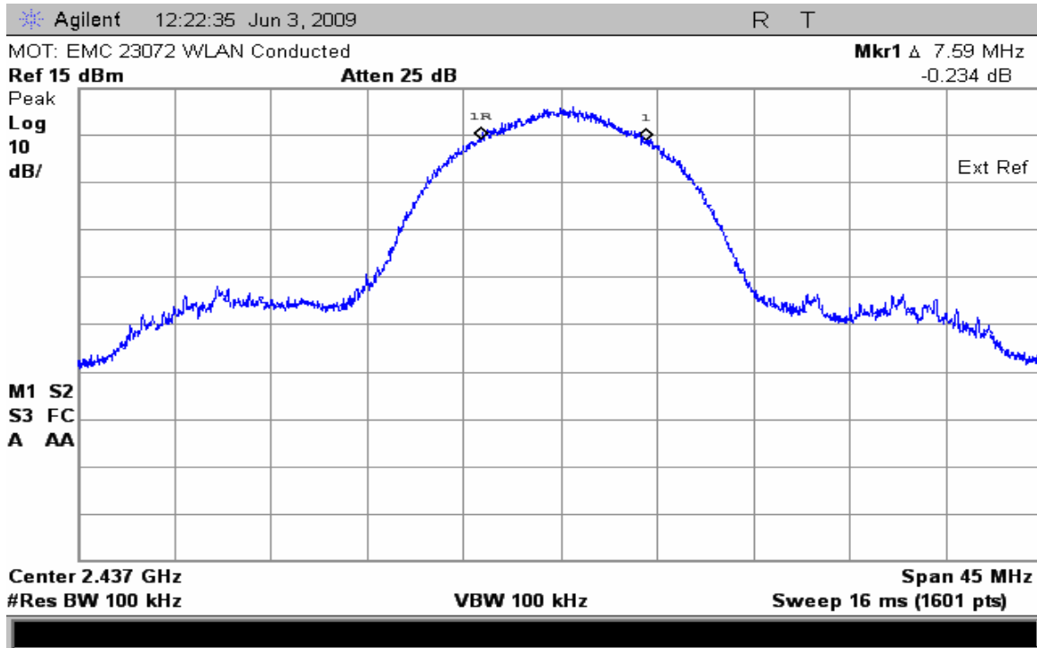
6dB Bandwidth Channel 6 @ 11 Mbps
