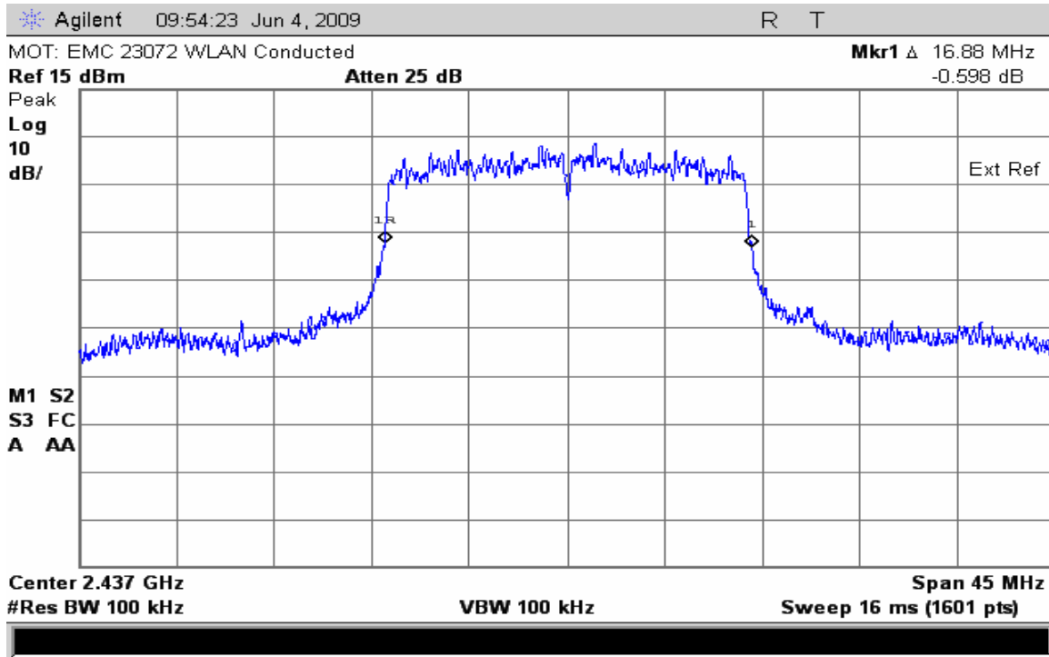
20dB Bandwidth Channel 6 @ 54 Mbps
