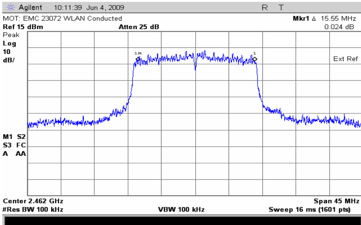
6dB Bandwidth Channel 11 @ 54 Mbps
