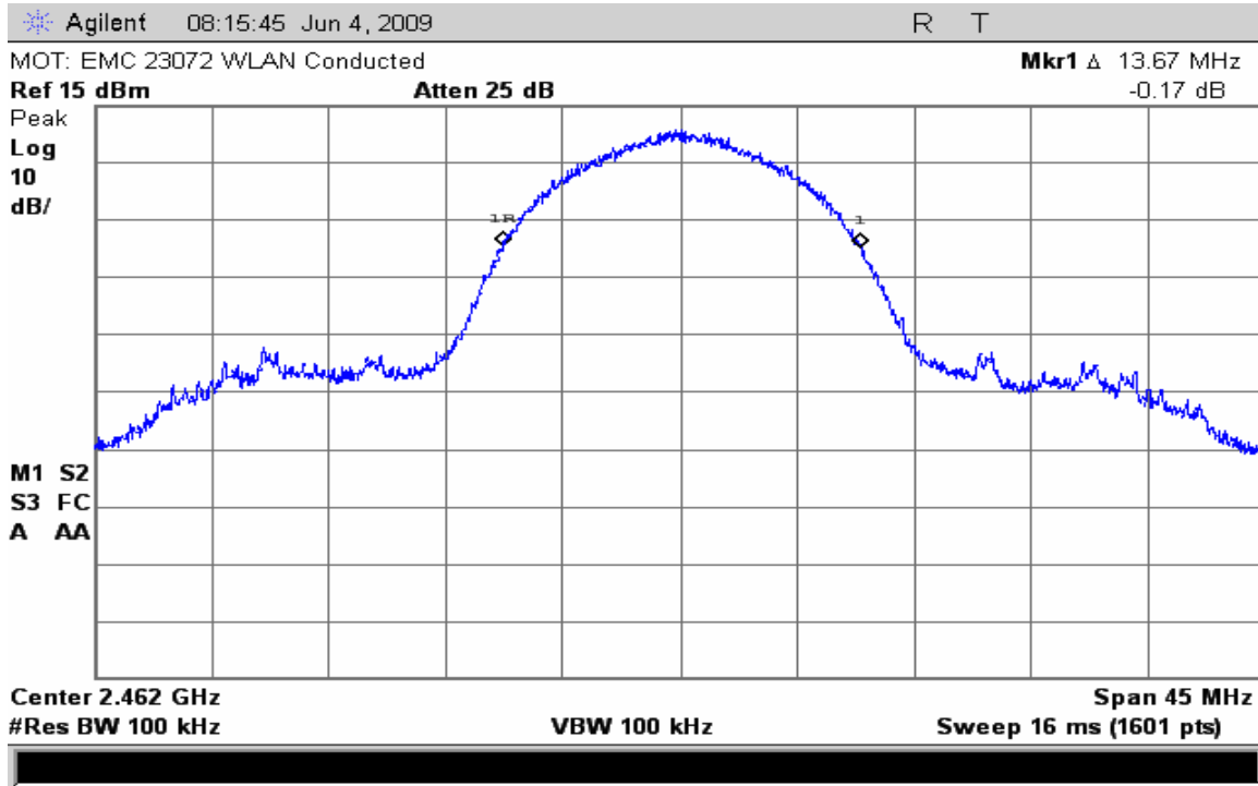
20dB Bandwidth Channel 11 @ 11 Mbps
