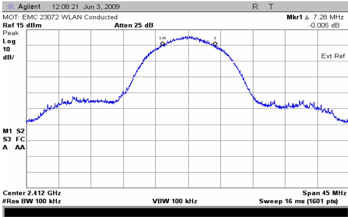
6dB Bandwidth Channel 1 @ 11 Mbps
