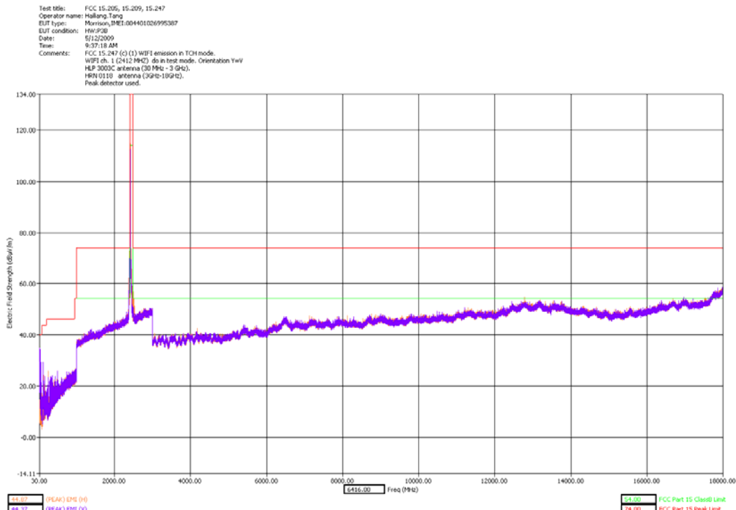
30 - 18000MHz Low Channel Dual Polarization Y - slider closed
