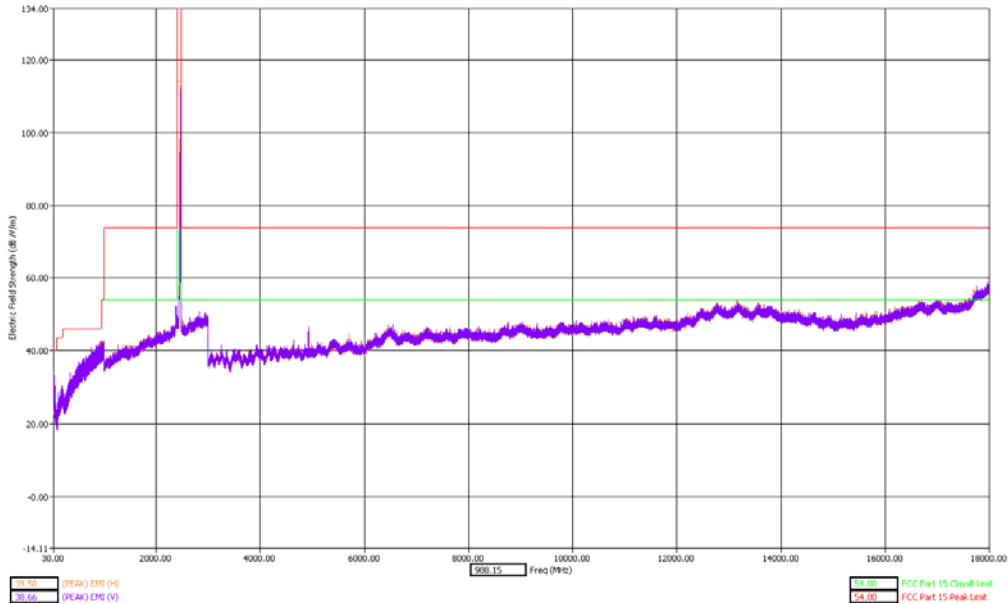
30 - 18000MHz High Channel Dual Polarization X - slider open
