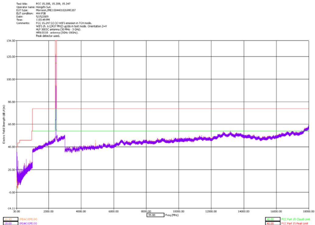
30 - 18000MHz Middle Channel Dual Polarization Z - slider open
