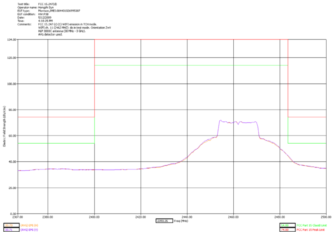
High Band Edge Z Orientation – slider closed
