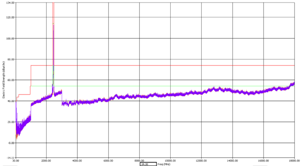
30 - 18000MHz High Channel Dual Polarization Z - slider closed
