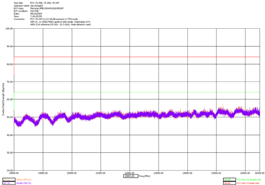
18-26.5GHz High Channel Z Orientation - slider closed
