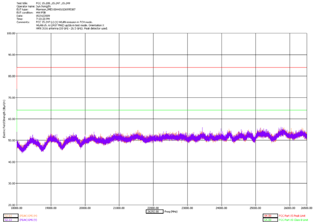
18-26.5GHz Middle Channel X Orientation - slider open
