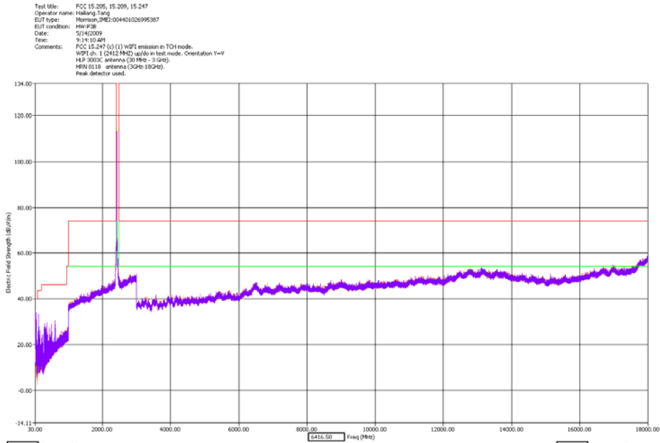
30 - 18000MHz Low Channel Dual Polarization X - slider open
