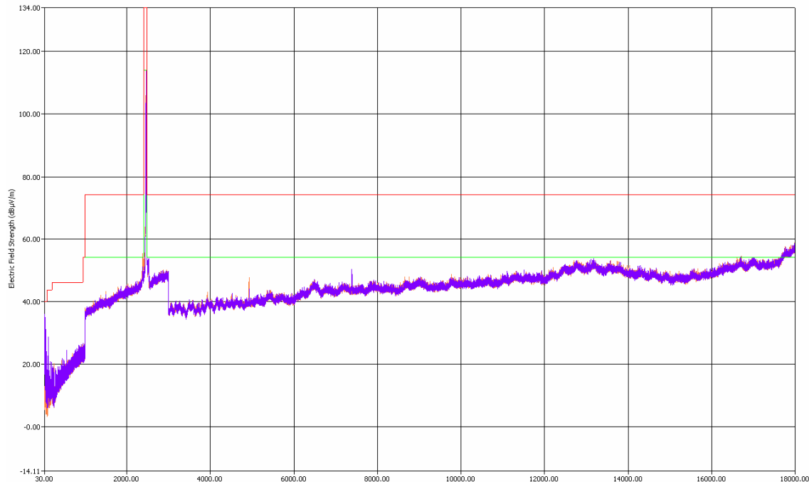
30 - 18000MHz High Channel Dual Polarization Z - slider closed
