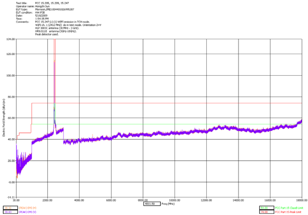
30 - 18000MHz Low Channel Dual Polarization Z - slider closed
