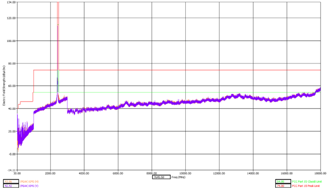
30 - 18000MHz Low Channel Dual Polarization X - slider closed
