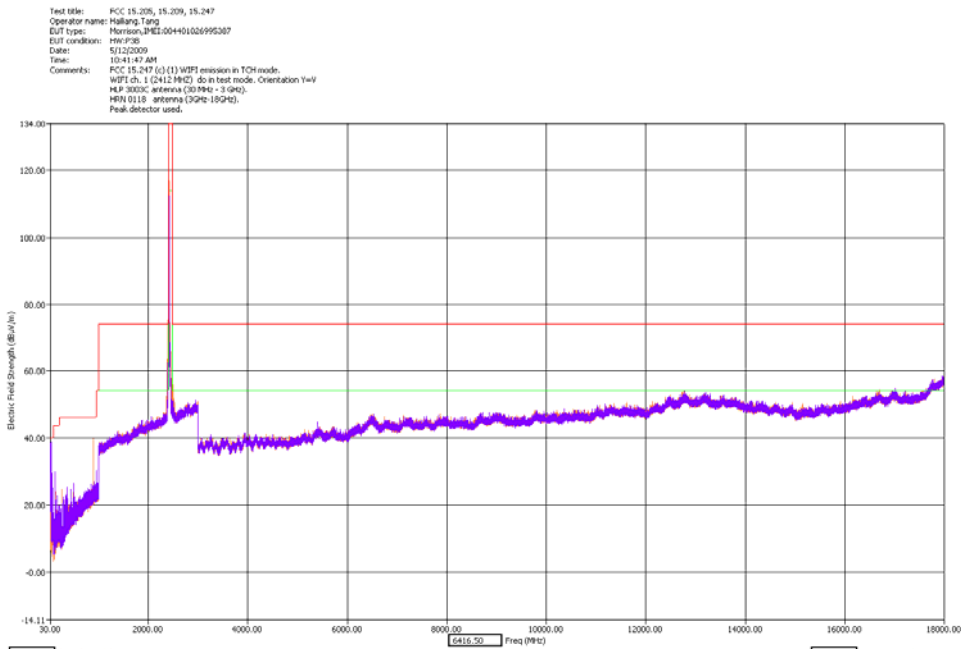
30 - 18000MHz Low Channel Dual Polarization X - slider closed
