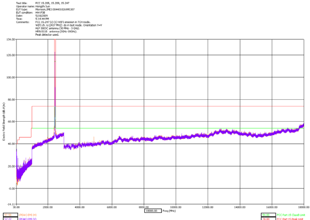
30 - 18000MHz Middle Channel Dual Polarization Y - slider closed
