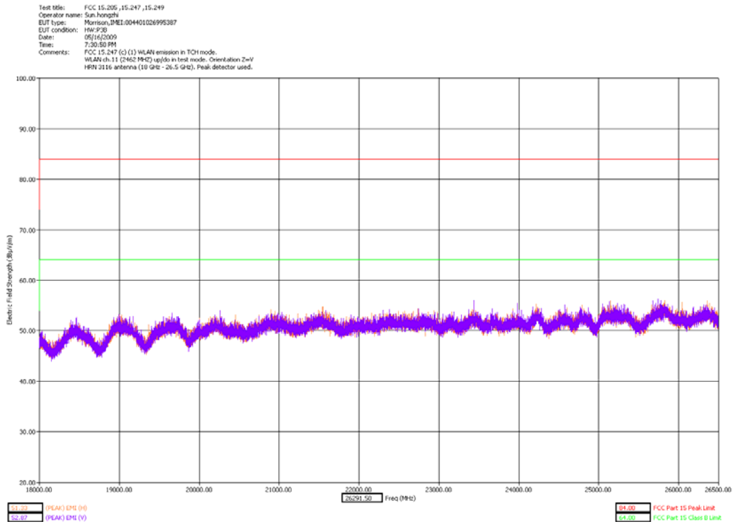
18-26.5GHz High Channel Z Orientation - slider open
