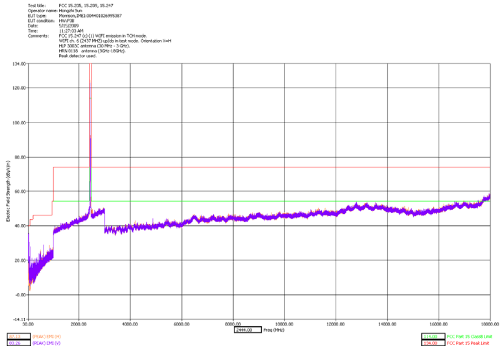
30 - 18000MHz Middle Channel Dual Polarization X - slider open
