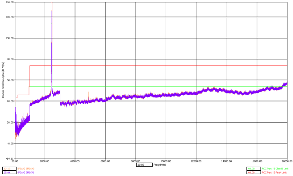
30 - 18000MHz Middle Channel Dual Polarization Z - slider closed
