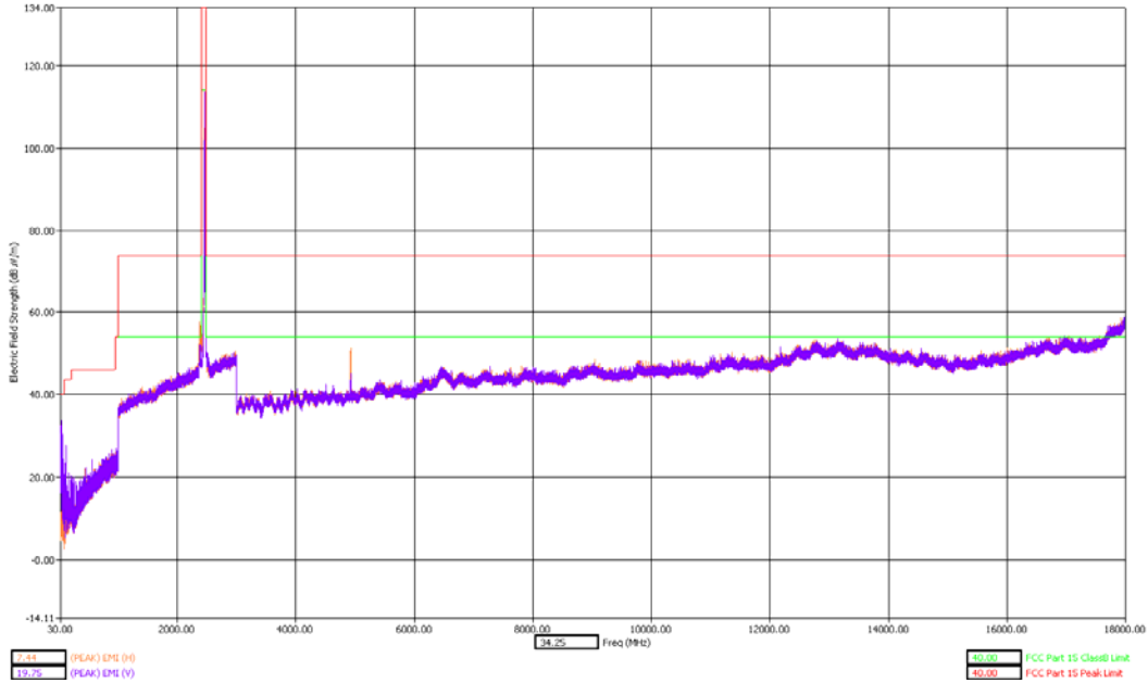
30 - 18000MHz High Channel Dual Polarization Y - slider closed
