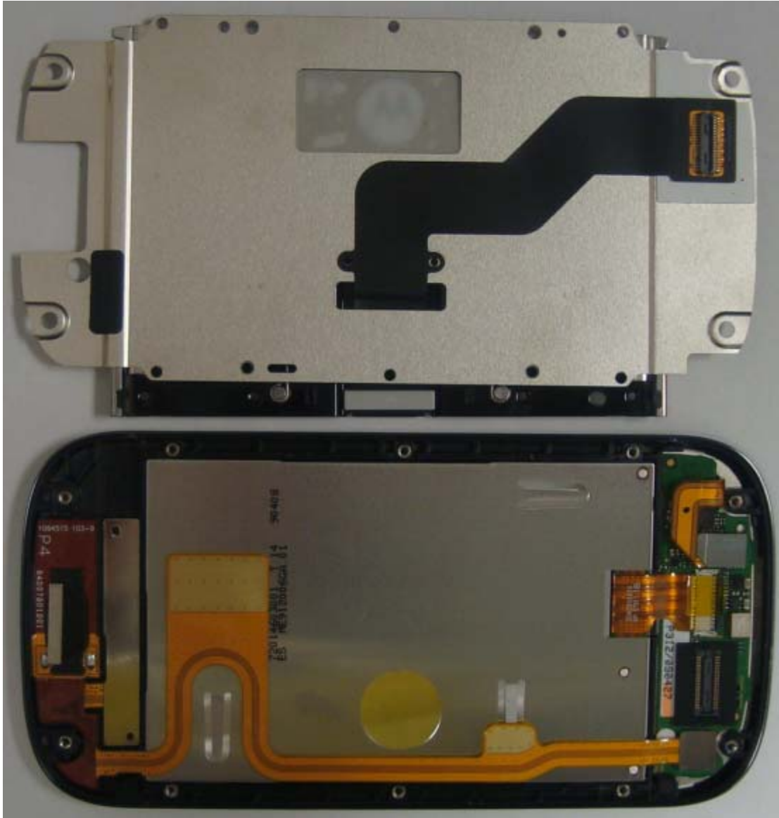
Inside of Slider
