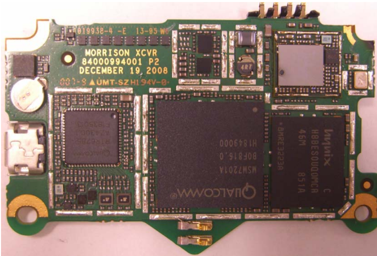
Main Board Bottom Without Shields
