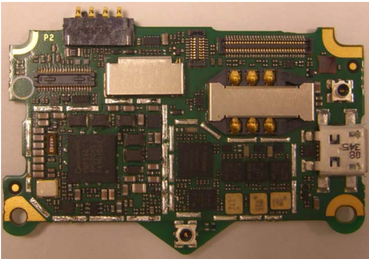
Main Board Top Without Shields
