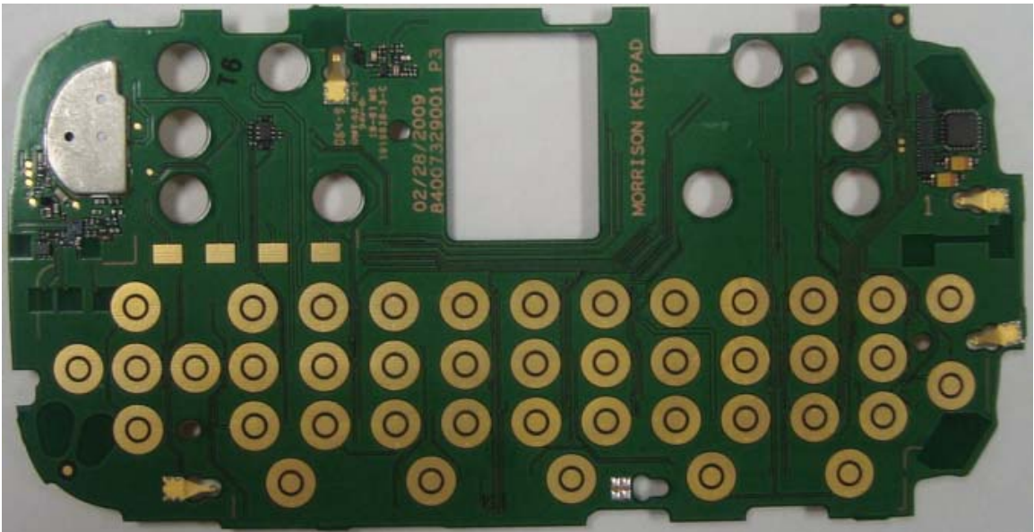
Top of Keypad board
