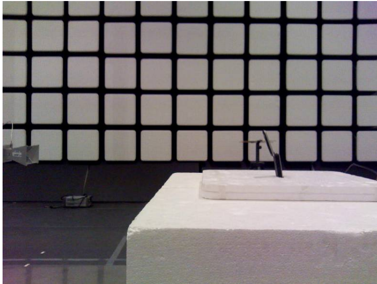
23145-1, IHDT56KS1 setup in semi-anechoic chamber – right view (18 GHz – 26.5 GHz)
