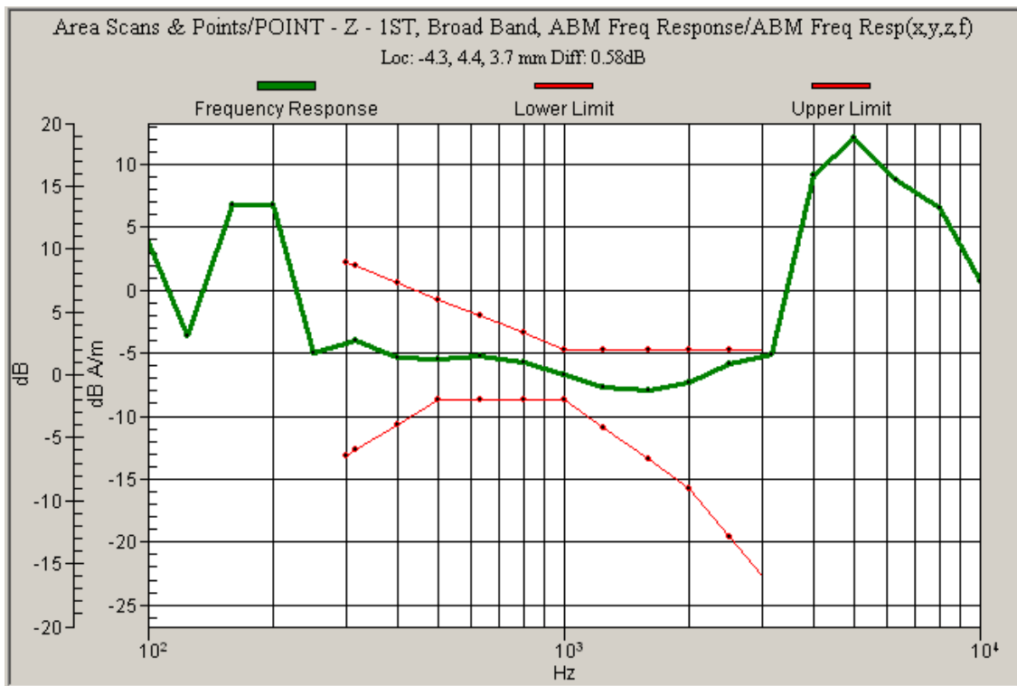
Graph 9: CDMA 1700 Frequency Response with Battery 4
