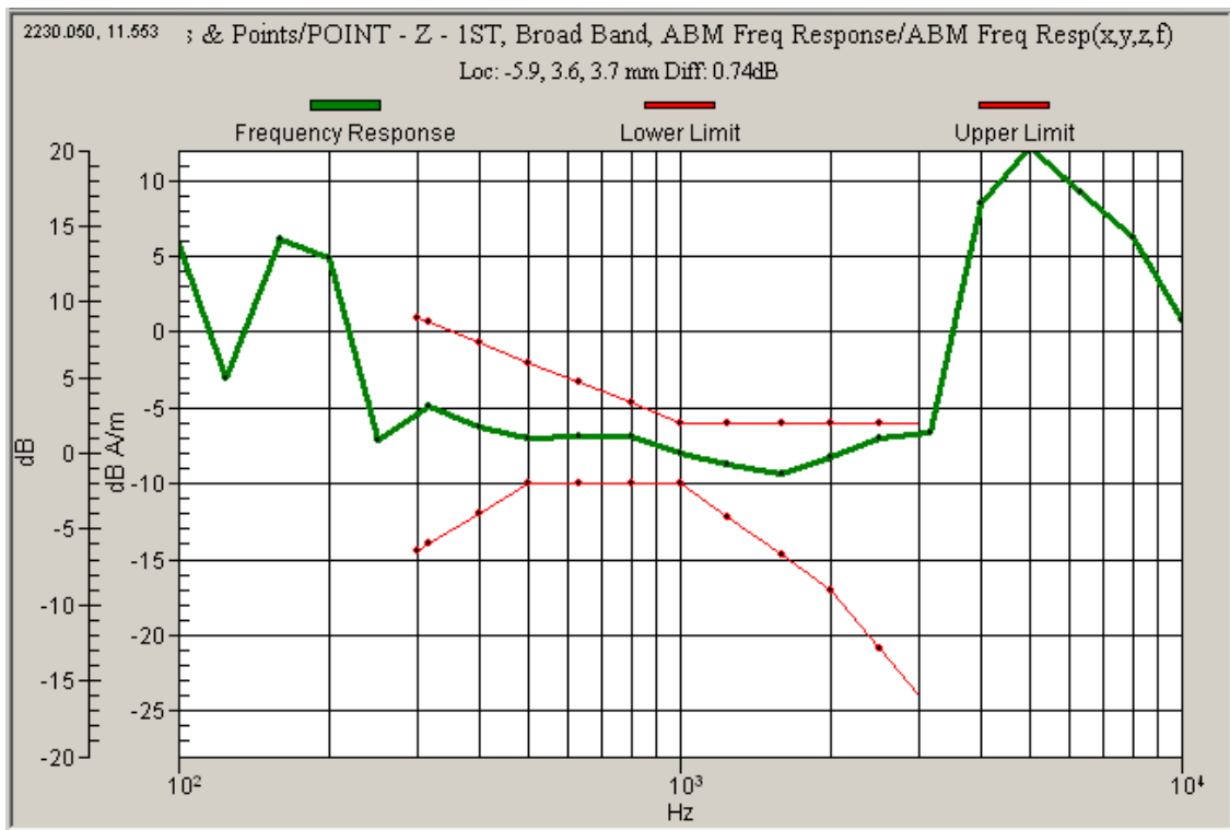
Graph 11: CDMA 1900 Frequency Response with Battery 2
