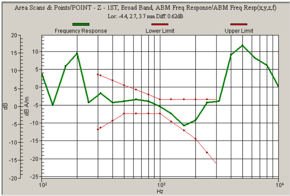
Graph 12: CDMA 1900 Frequency Response with Battery 3
