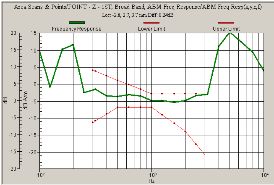
Graph 8: CDMA 1700 Frequency Response with Battery 3
