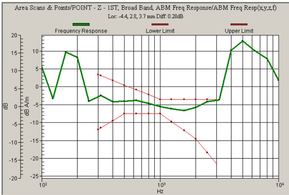
Graph 13: CDMA 1900 Frequency Response with Battery 4
