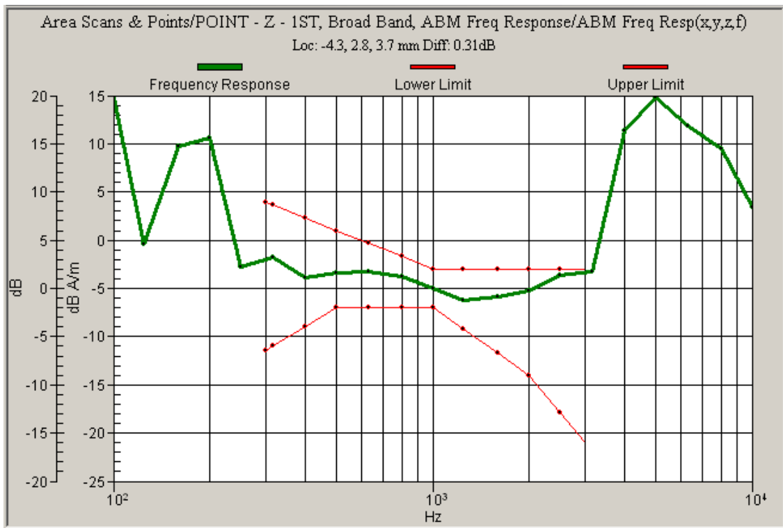
Graph 7: CDMA 1700 Frequency Response with Battery 2
