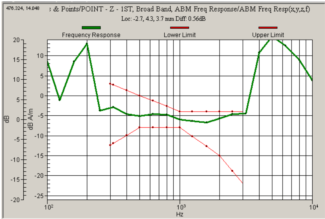
Graph 10: CDMA 1900 Frequency Response
