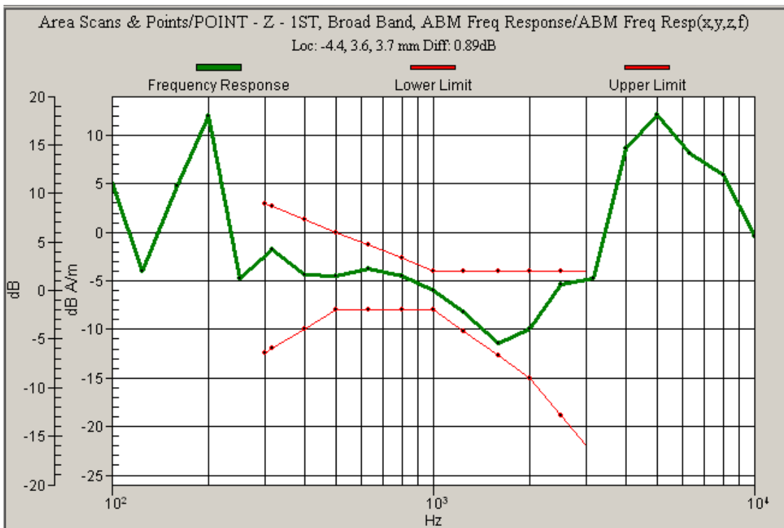
Graph 5: CDMA 800 Frequency Response with Battery 4
