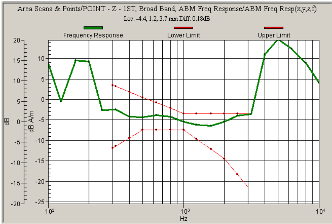
Graph 6: CDMA 1700 Frequency Response
