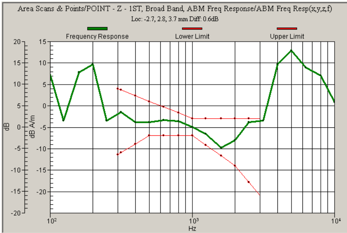
Graph 4: CDMA 800 Frequency Response with Battery 3
