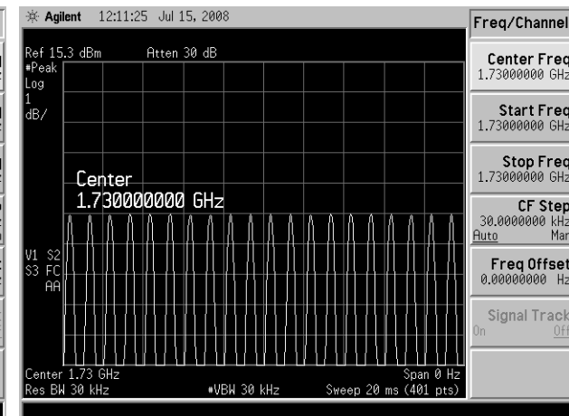
80% AM 1730 MHz
