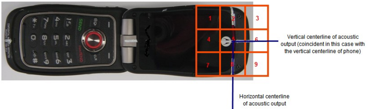
Figure 5. Phone Open - Orientation and Measurement Plane for RF Emissions Testing
