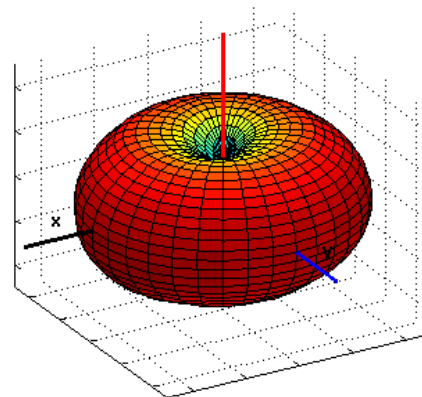
Figure 6b.5-2 Antenna pattern in the 900 MHz ISM frequency band (Flip Closed).
