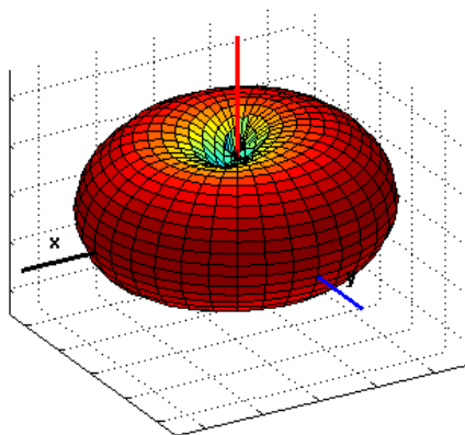
Figure 6b.5-1 Antenna pattern in the 900 MHz ISM frequency band (Flip Open).
