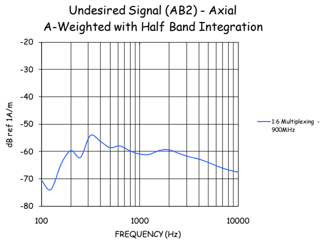
Figure 9-4-2: 900 MHz Undesired Signal (1:6).
