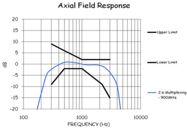
Figure 9-1-3: 900 MHz Measured Frequency Response (2:6).
