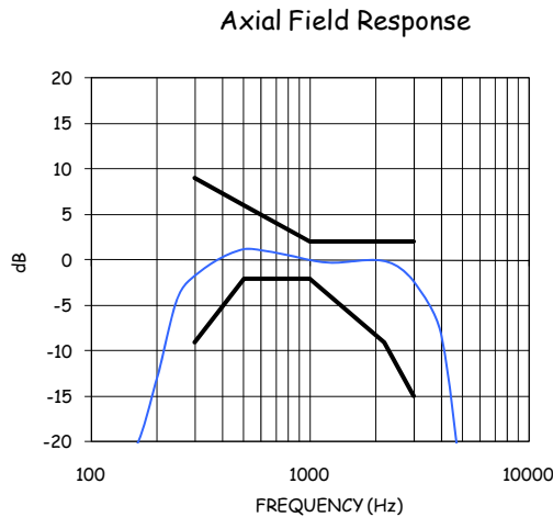
Figure 9-1-1: 800 MHz Measured Frequency Response (2:6).
