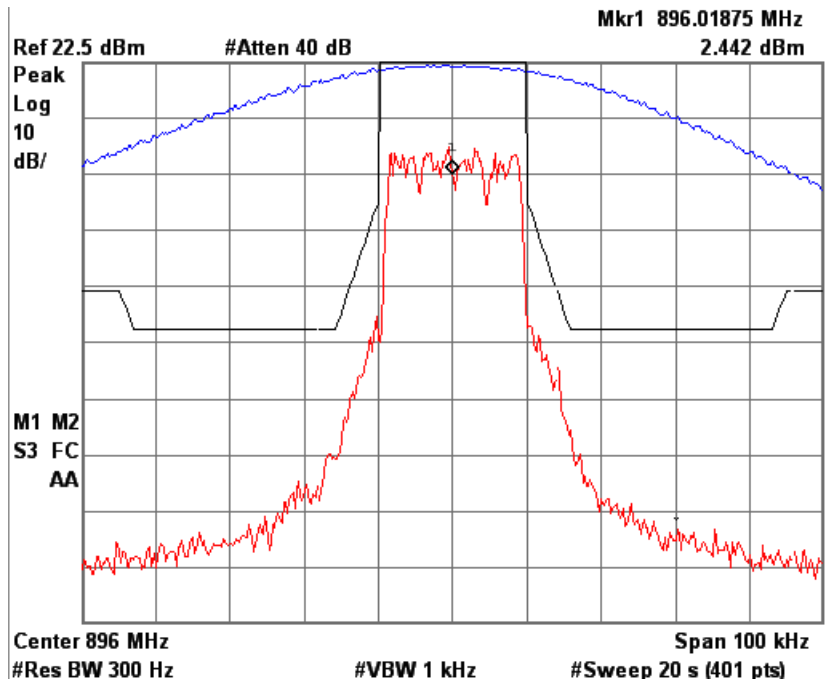
Figure 6a-2.2.9. iDEN 900 MHz Band, QAM64, Maximum Power, Emission Mask G
