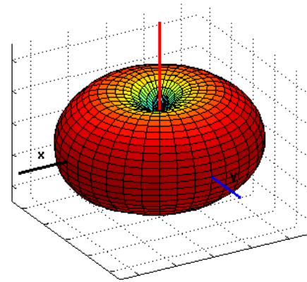
Figure 6a.6-6 Antenna pattern in the 900 MHz NBPCS frequency band (Flip Closed).
