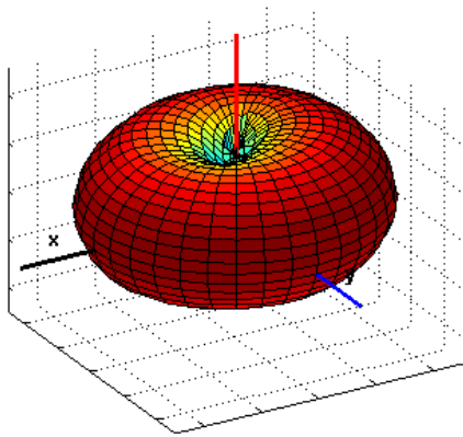
Figure 6a.6-5 Antenna pattern in the 900 MHz NBPCS frequency band (Flip Open).
