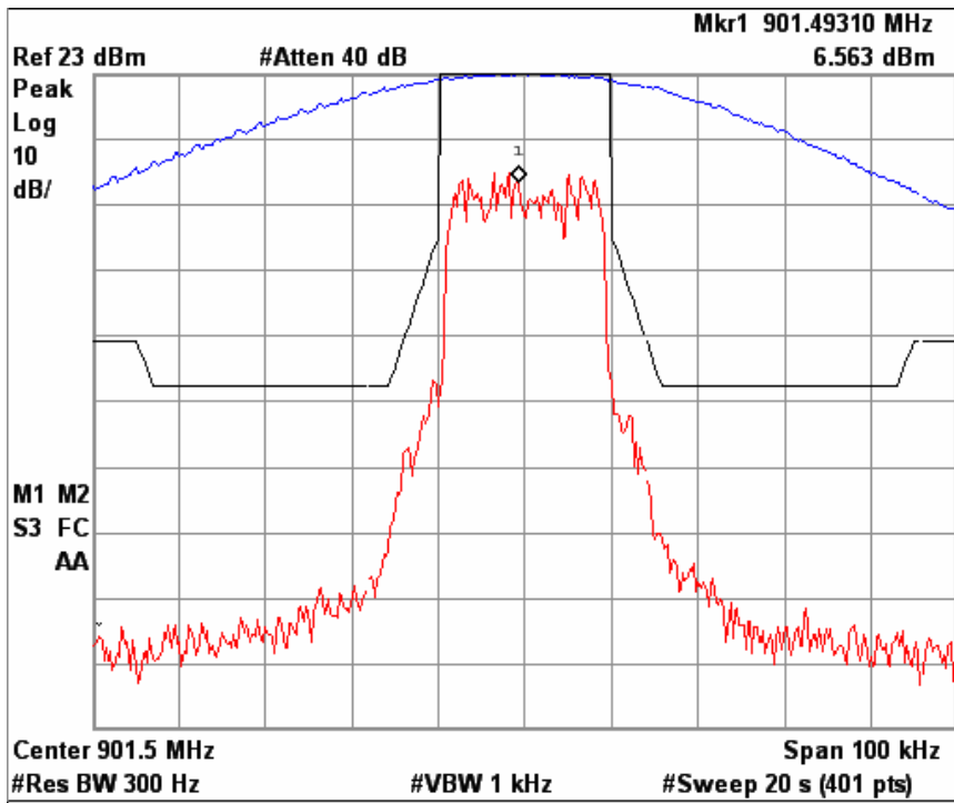
Figure 6b.2.1-3 iDEN NBPCS Band, Occupied Bandwidth, Quad-64QAM, Maximum Power.
