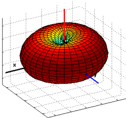
Figure 6a.6-3 Antenna pattern in the 900 MHz SMR frequency band (Flip Open).
