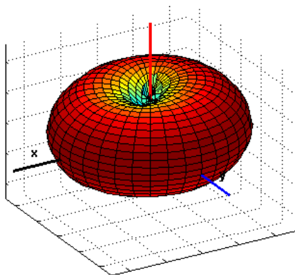
Figure 6a.6-1 Antenna pattern in the 800 MHz SMR frequency band (Flip Open).
