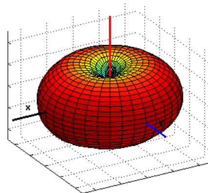
Figure 6a.6-2 Antenna pattern in the 800 MHz SMR frequency band (Flip Closed).
