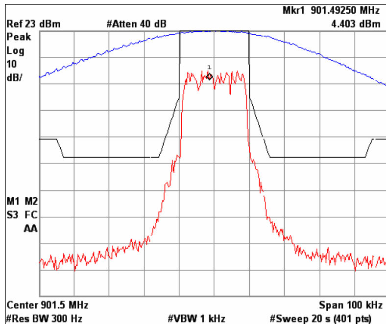
Figure 6b.2.1-2 iDEN NBPCS Band, Occupied Bandwidth, Quad-16QAM, Maximum
