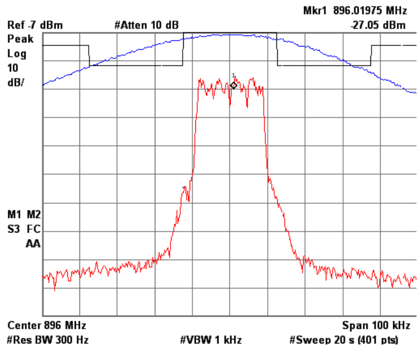
Figure 6a-2.2.12. iDEN 900 MHz Band, QAM64, Minimum Power, EA Emission Mask
