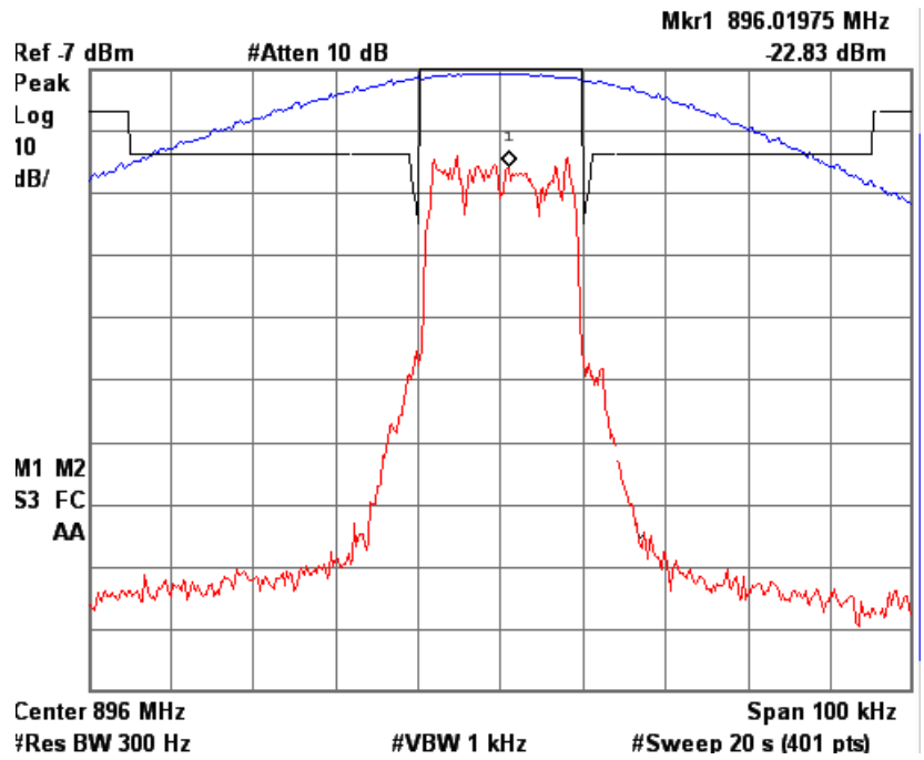
Figure 6a-2.2.10. iDEN 900 MHz Band, QAM64, Minimum Power, Emission Mask G
