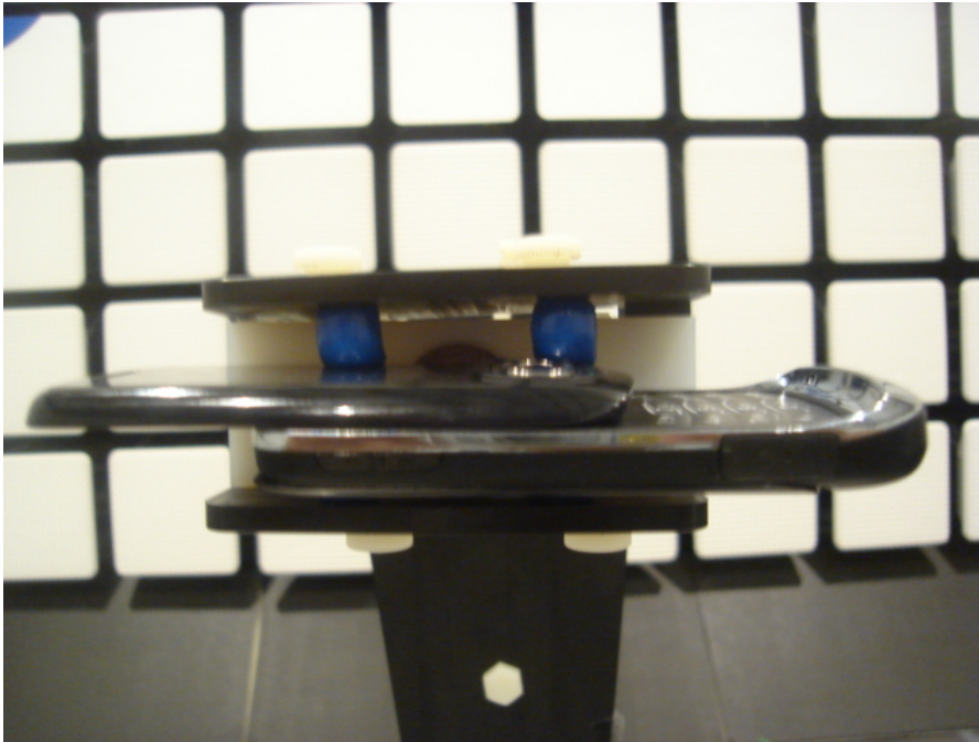
22719-1, IHDT6KP3 placed in test position X – slider open
