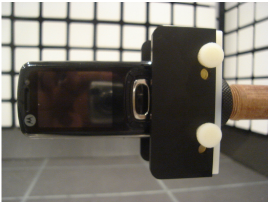
22719-1, IHDT6KP3 placed in test position Y – slider closed
