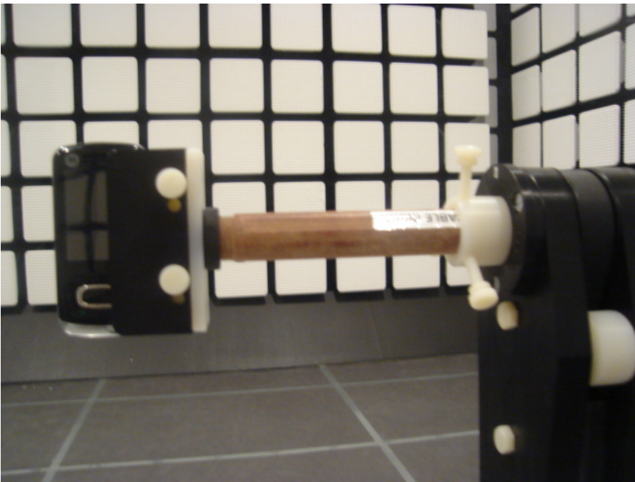
22719-1, IHDT6KP3 placed in test position Z – slider closed
