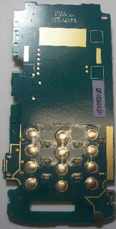
Front View with Keypad Popple (Shields Removed)
