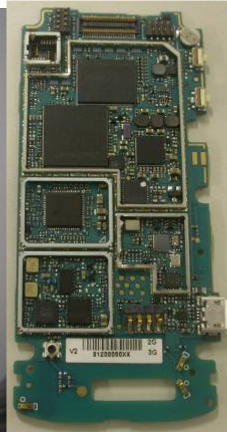
Rear View (Shields Removed)
