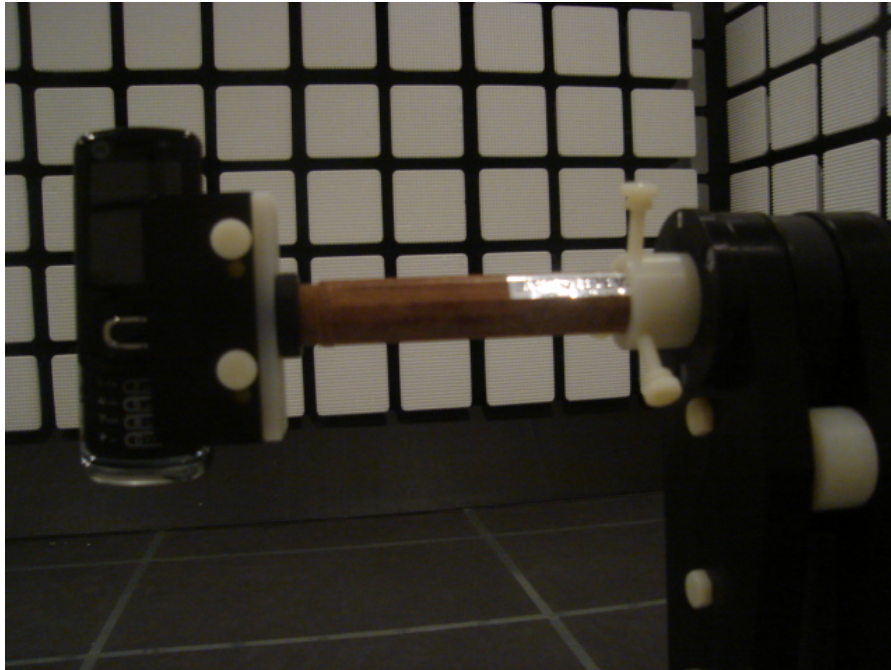
22718-1, IHDT56KP2 placed in test position Z – slider open
