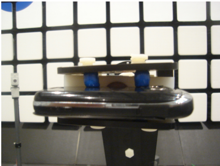
22718-1, IHDT56KP2 placed in test position X – slider closed
