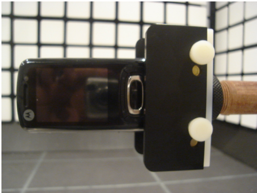
22718-1, IHDT56KP2 placed in test position Y – slider closed
