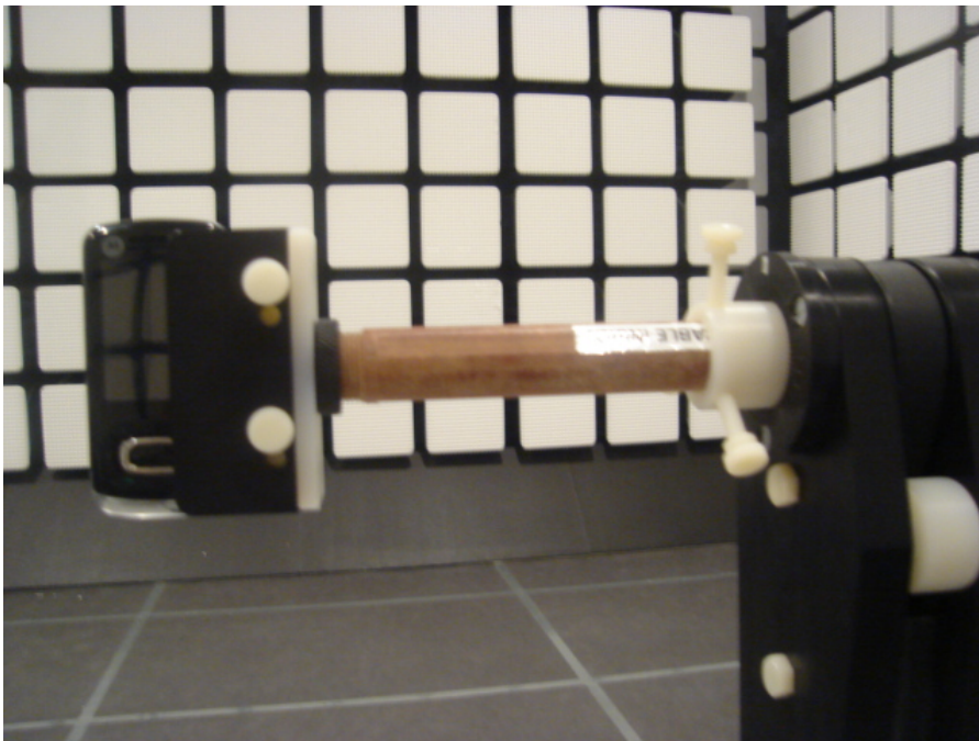
22718-1, IHDT56KP2 placed in test position Z – slider closed
