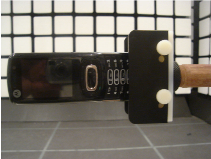
22718-1, IHDT56KP2 placed in test position Y – slider open
