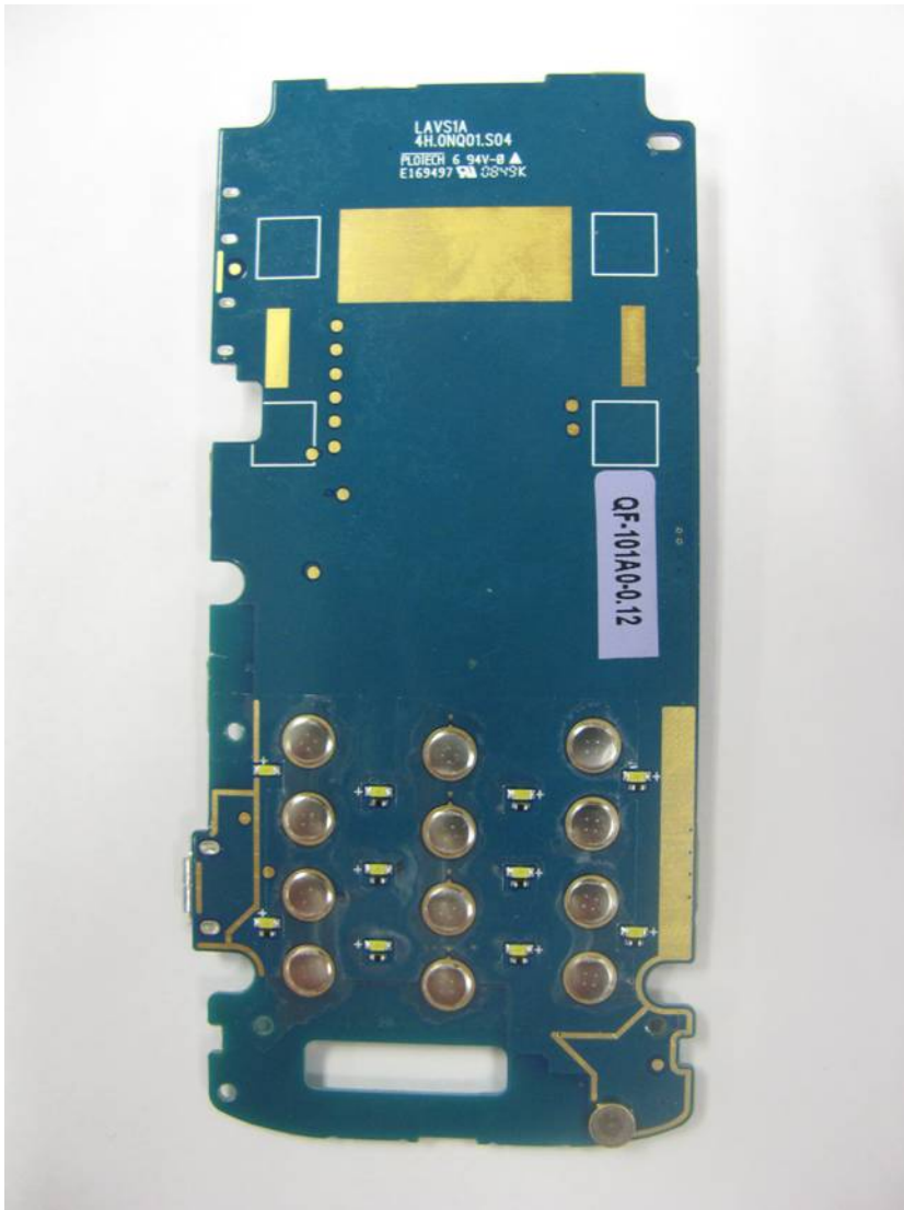
Front View with Keypad Popple (Shields Removed)
