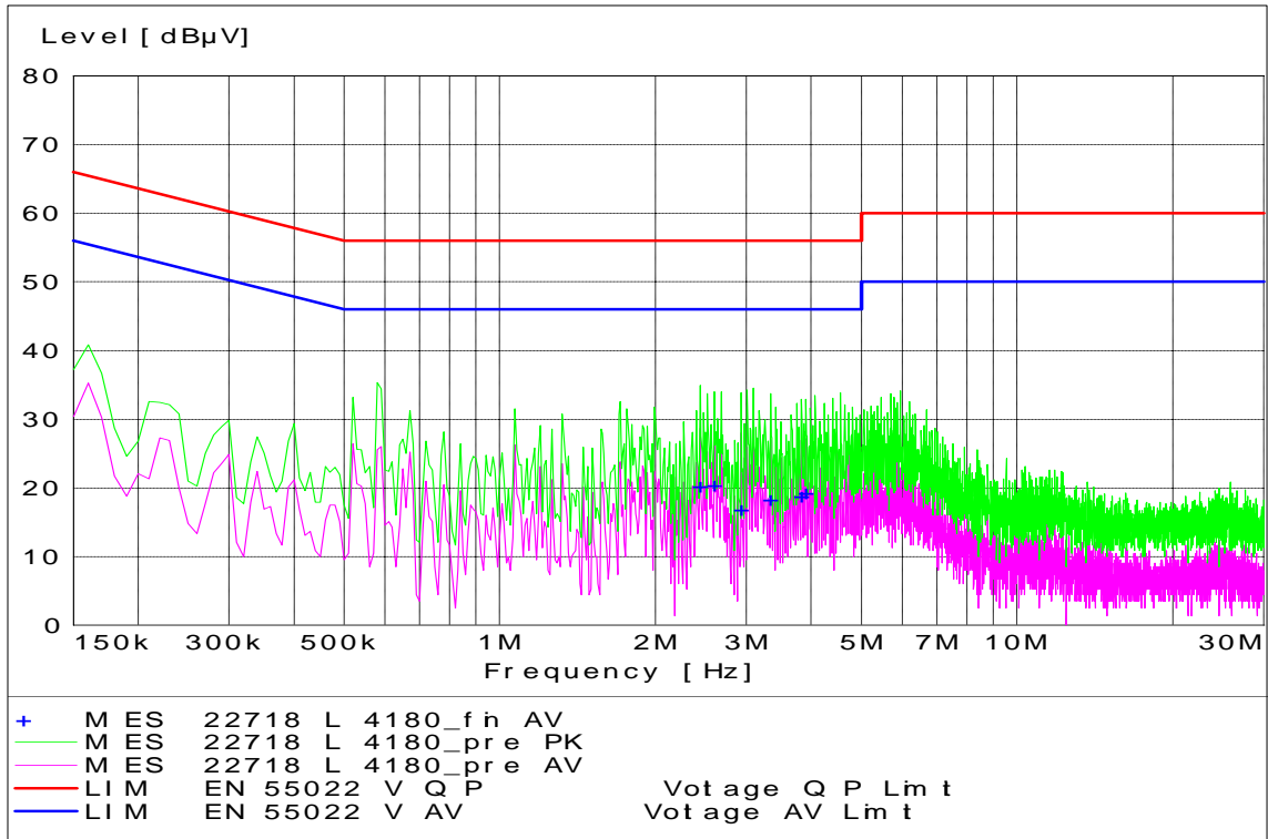
WCDMA Channel 4180 - Tx Mode - Line Coupling
