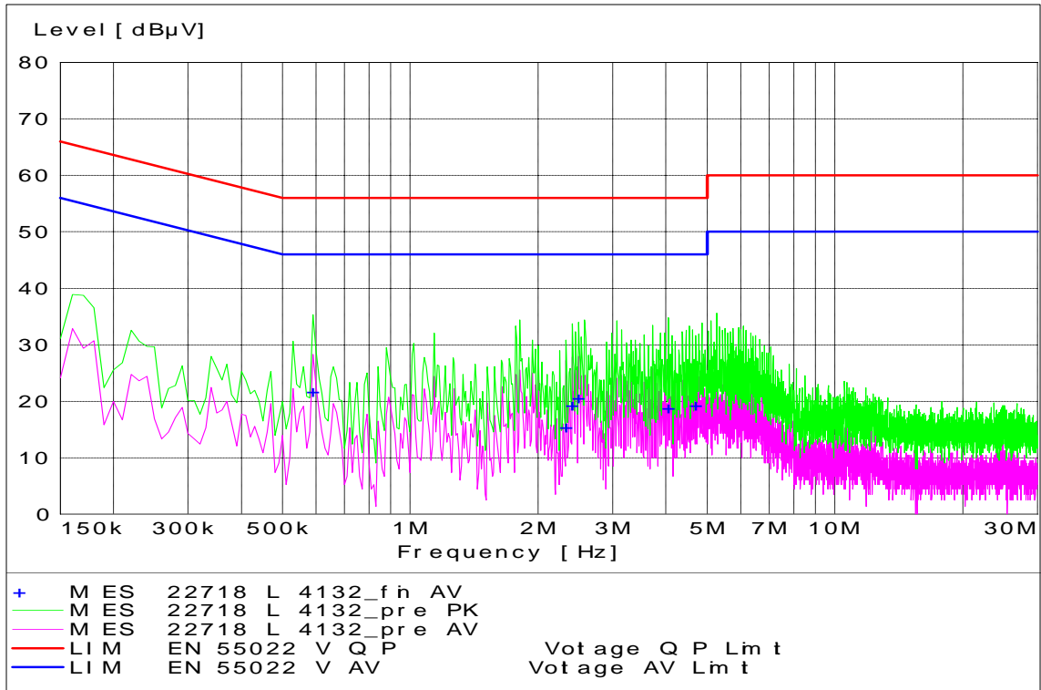
WCDMA Channel 4132 - Tx Mode – Line Coupling
