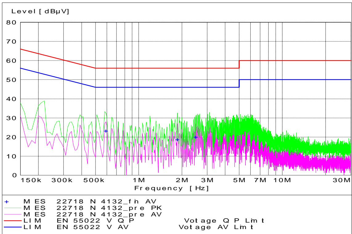
WCDMA Channel 4132 - Tx Mode - Neutral Coupling
