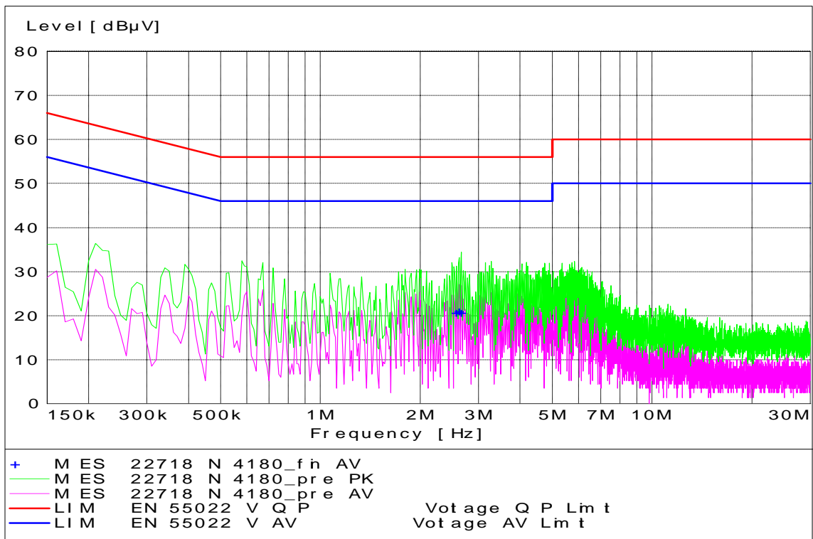
WCDMA Channel 4180 - Tx Mode - Neutral Coupling
