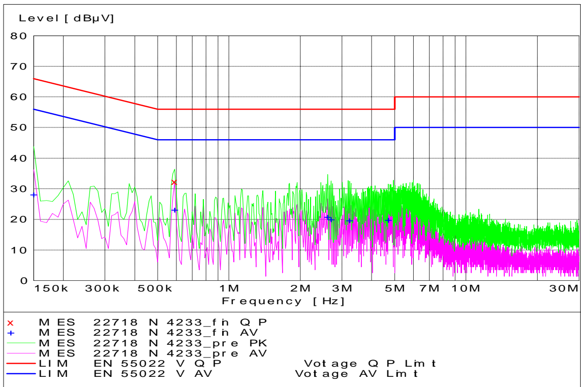
WCDMA Channel 4233 - Tx Mode - Neutral Coupling
