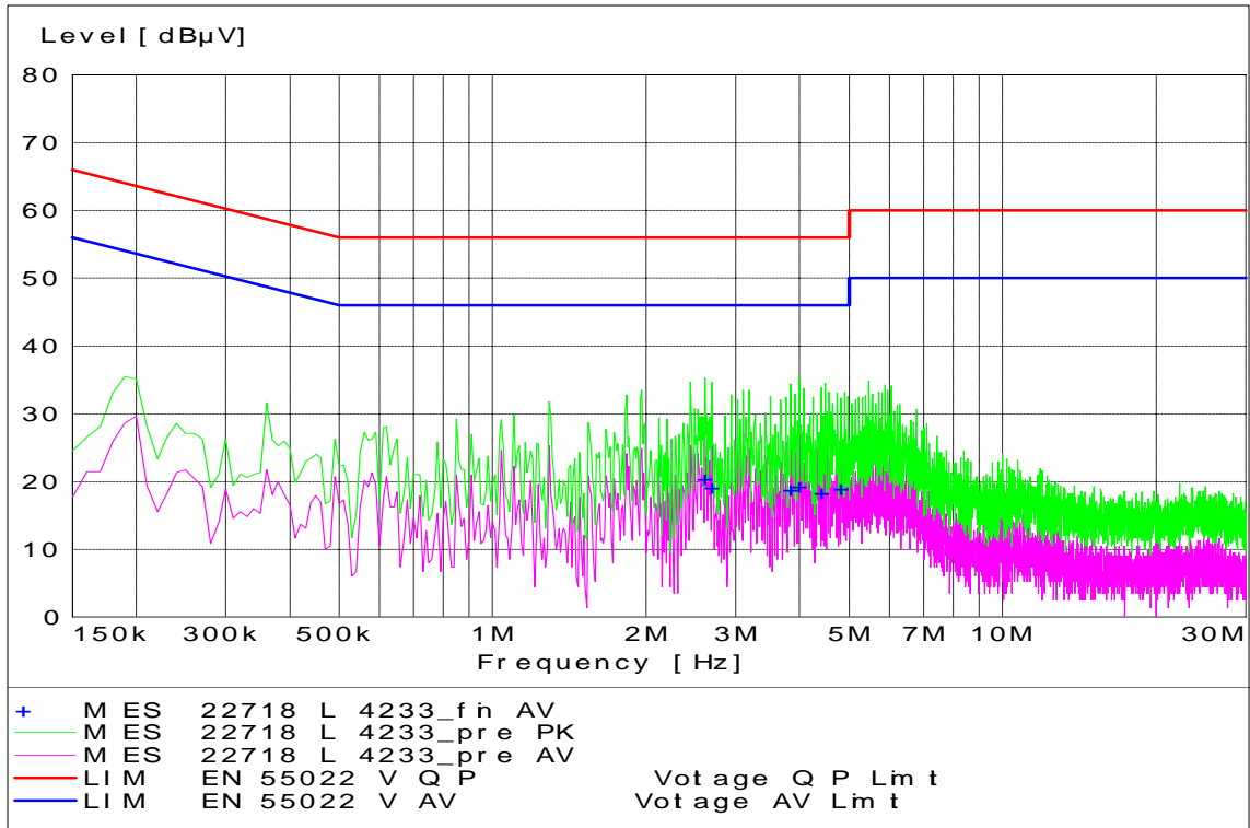
WCDMA Channel 4233 - Tx Mode - Line Coupling
