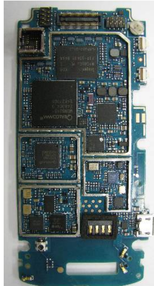
Rear View (Shields Removed)
