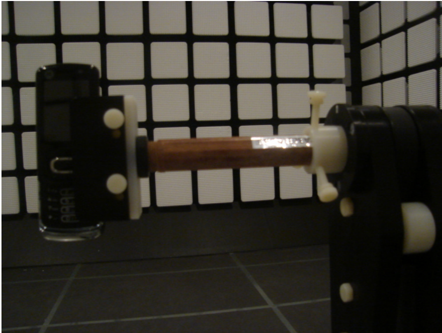
22874-1, IHDT56KP1 placed in test position Z – slider open
