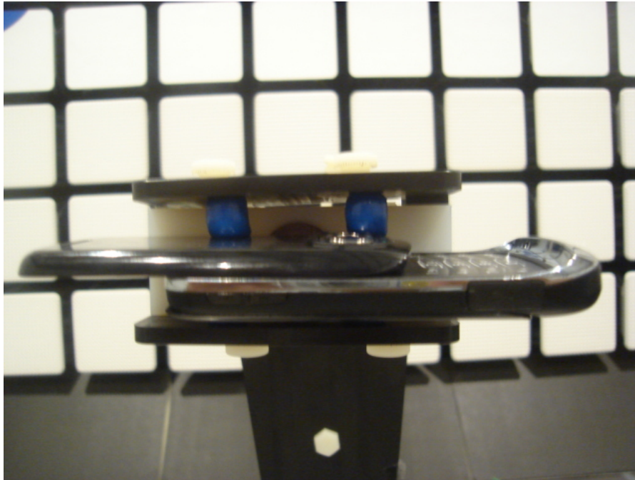
22874-1, IHDT56KP1 placed in test position X – slider open
