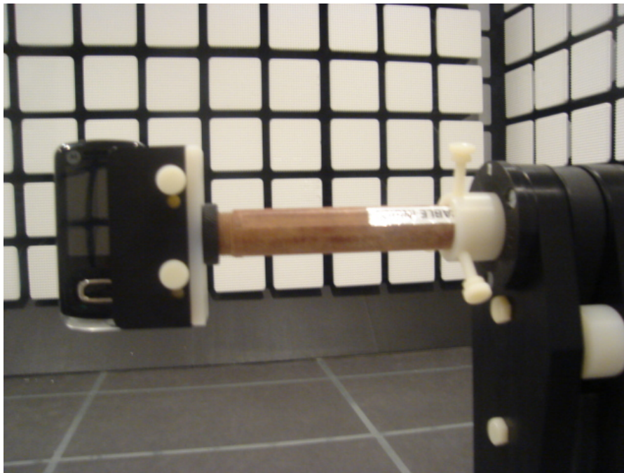
22874-1, IHDT56KP1 placed in test position Z – slider closed
