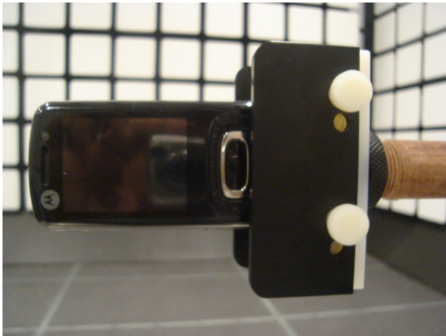
22874-1, IHDT56KP1 placed in test position Y – slider closed
