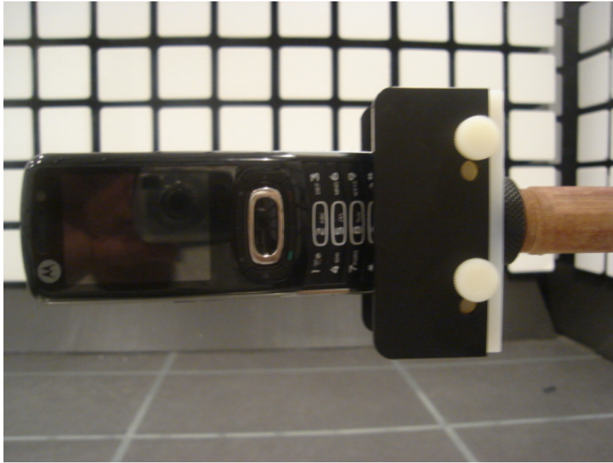
22874-1, IHDT56KP1 placed in test position Y – slider open
