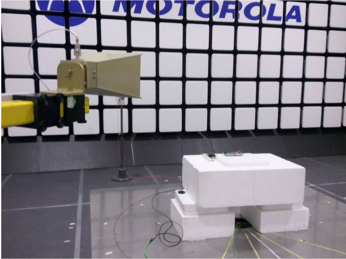
Radiated Emissions
