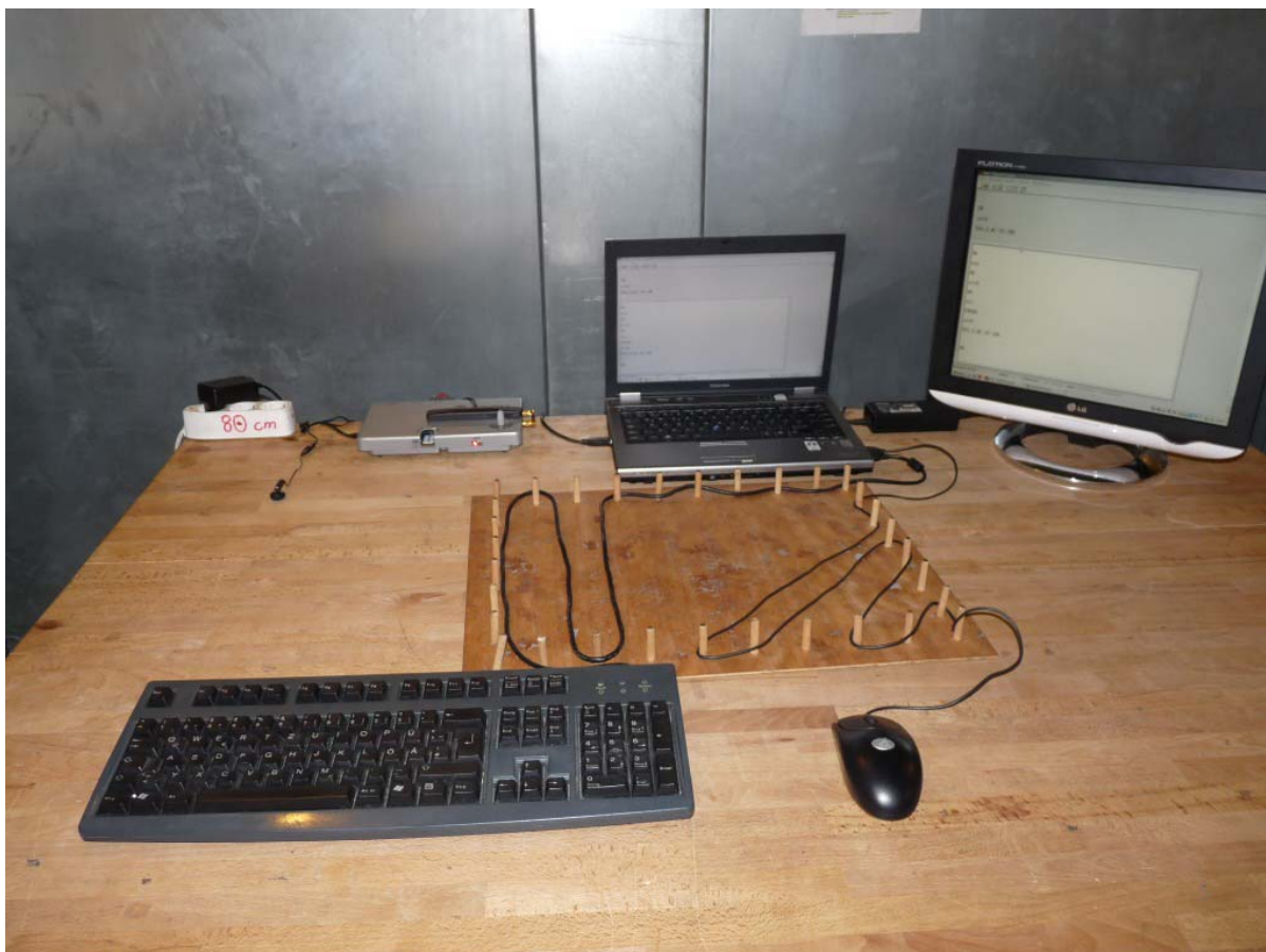
Setup for conducted emissions AC mains
