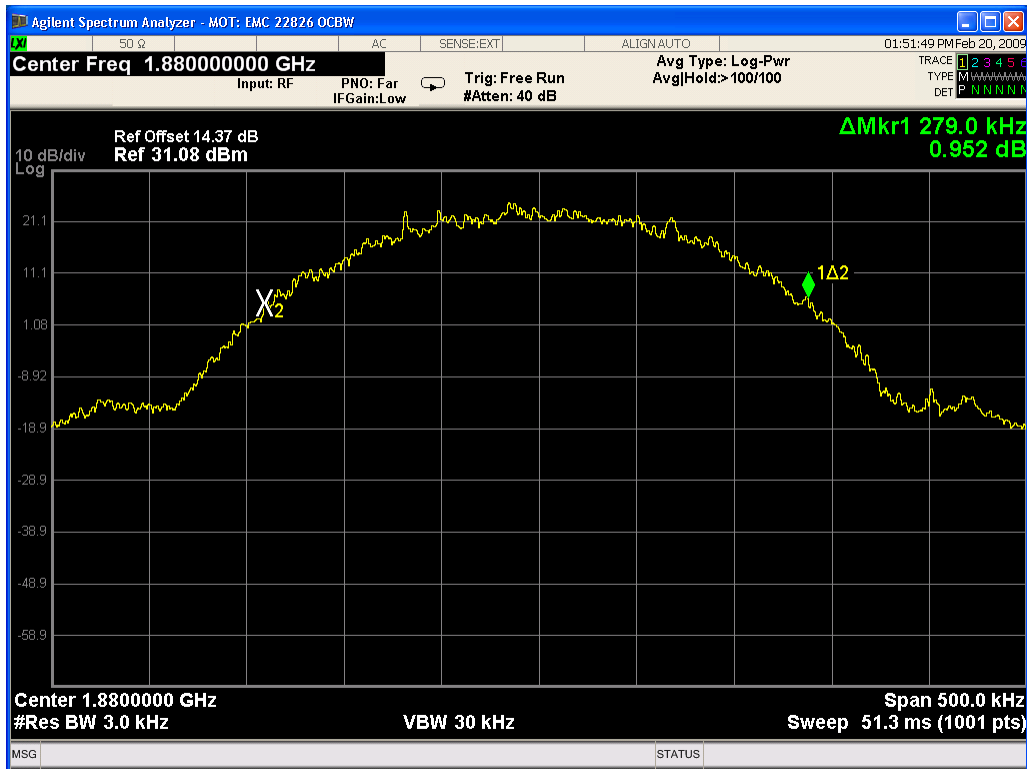
GSM 1900 – Occupied Bandwidth – Channel 661 (1880.00MHz)
