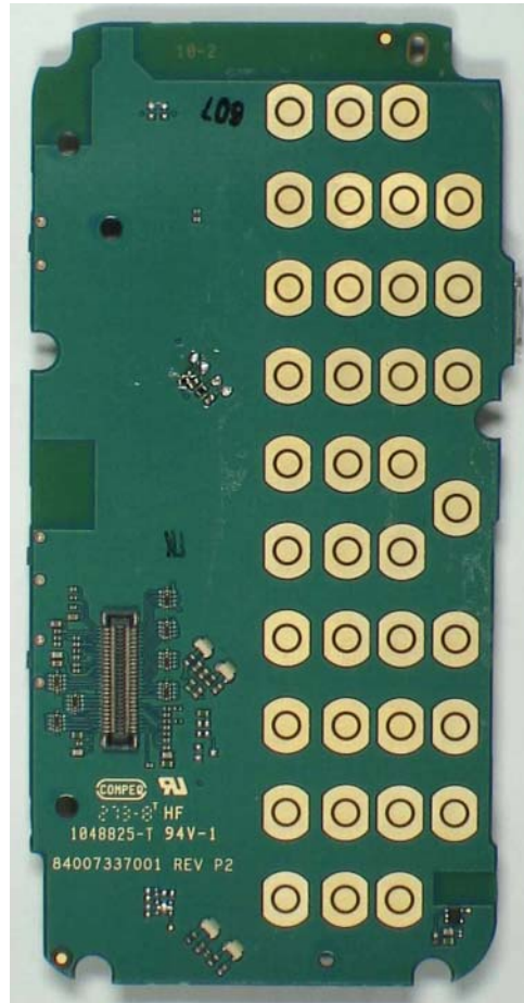
Main Board Top Without Popples
