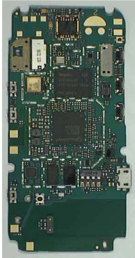
Main Board bottom Without Shields
