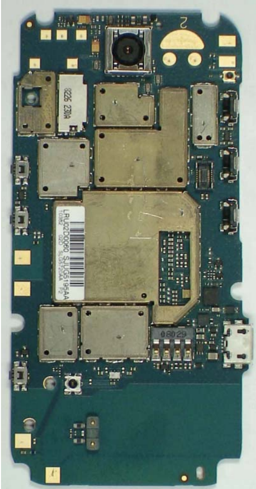
Main Board bottom With Shields
