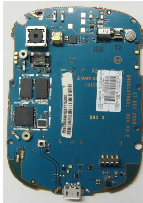
Main Board Bottom Without Shields
