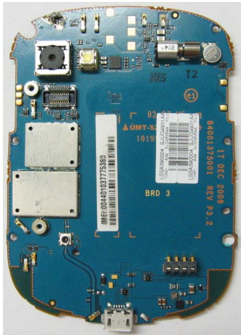
Main Board Bottom With Shields
