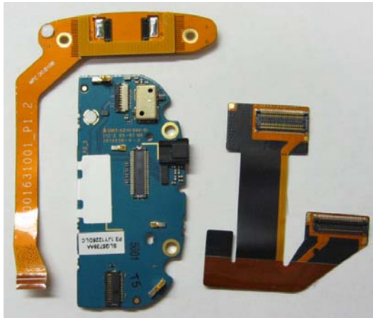
Slide PCB with Shields & Slide Flexes
