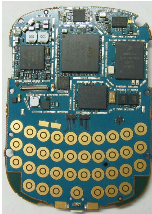
Main Board Top Without Popples or Shields
