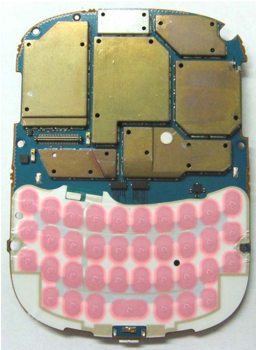
Main Board Top With Shields
