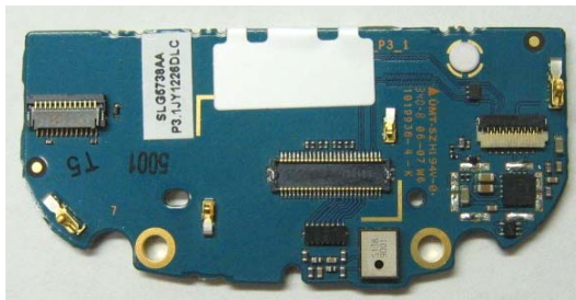
Slide PCB Without Shields
